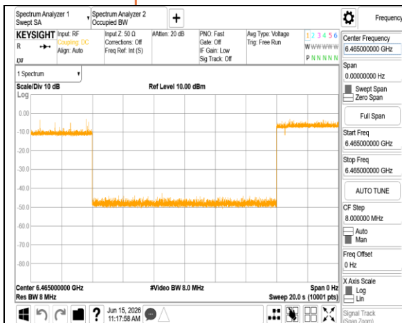
ax 80M_6465MHz_Int6465MHz_-77.11dBm_OFF
