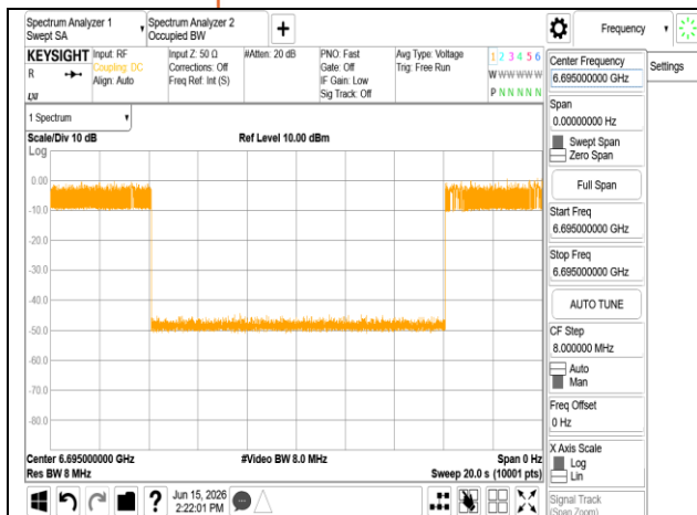
ax 20M 6695MHz Int6695MHz -77.15dBm OFF
