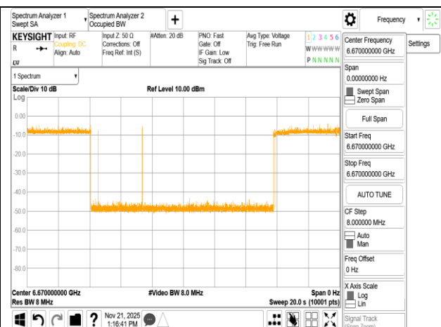
ax 80M_6705MHz_Int6670MHz_-76.68dBm Minimal
