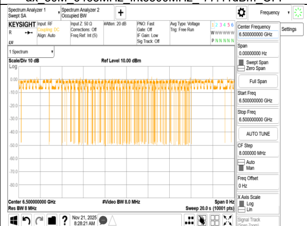
ax 80M_6465MHz_Int6500MHz_-79.41dBm ON
