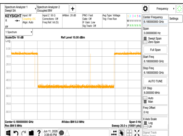
ax 80M 6145MHz Int6180MHz -77.11dBm Minimal
