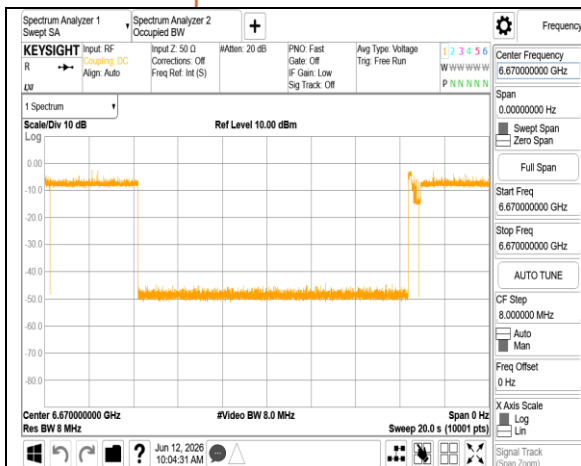
ax_80M_6705MHz_Int6670MHz_-75.07dBm OFF
