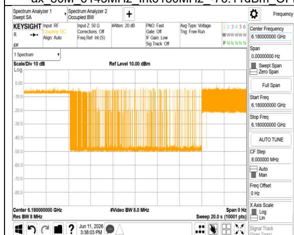
ax 80M 6145MHz Int6180MHz -78.11dBm ON
