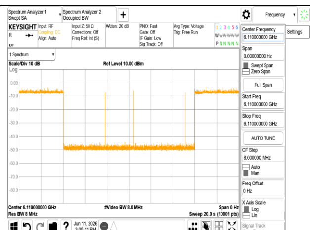
ax 80M 6145MHz Int6110MHz -77.1dBm Minimal
