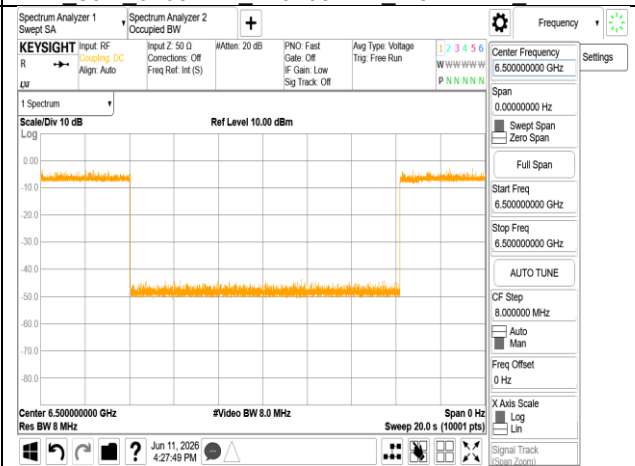
ax 80M_6465MHz_Int6500MHz_-75.14dBm_OFF
