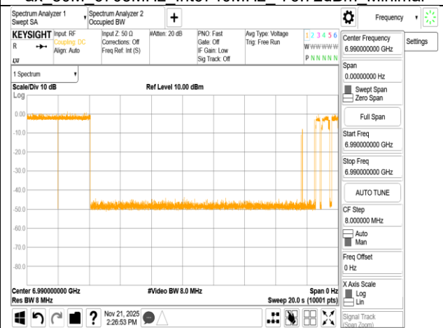
ax_80M_7025MHz_Int6990MHz_-76.62dBm OFF
