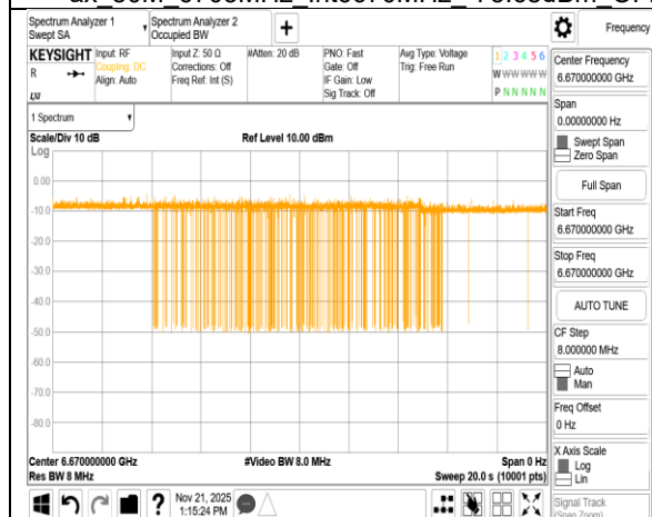
ax 80M_6705MHz_Int6670MHz_-77.68dBm ON
