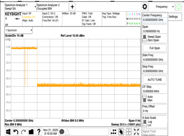
ax 80M_6465MHz_Int6500MHz_-77.41dBm OFF
