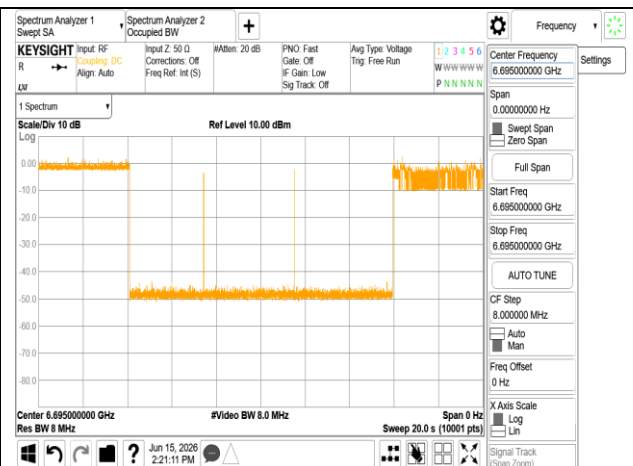
ax 20M 6695MHz Int6695MHz -78.15dBm Minimal
