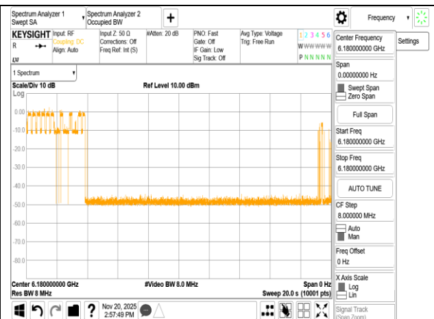
ax 80M 6145MHz Int6180MHz -78.47dBm Minimal
