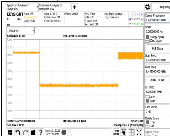
ax 80M_6465MHz_Int6465MHz_-69.47dBm OFF
