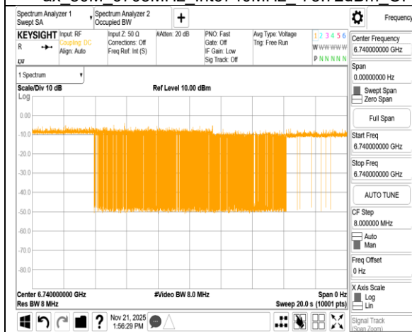
ax_80M_6705MHz_Int6740MHz_-77.72dBm ON
