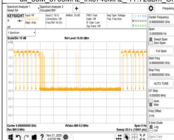
ax_80M_7025MHz_Int6990MHz_-77.62dBm Minimal
