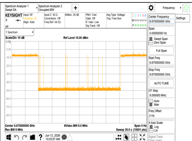
ax_80M_6705MHz_Int6670MHz_-75.57dBm Minimal
