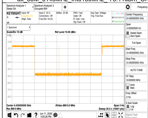
ax 80M 6465MHz Int6430MHz -76.12dBm Minimal
