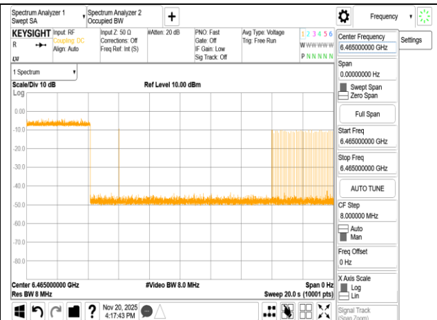
ax 80M_6465MHz_Int6465MHz_-70.47dBm Minimal
