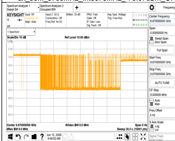
ax_80M_6705MHz_Int6670MHz_-76.07dBm ON
