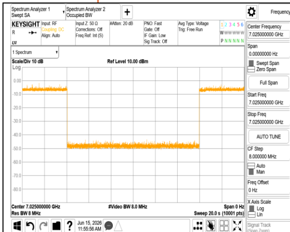
ax 80M 7025MHz Int7025MHz -75.01dBm OFF
