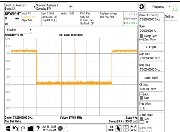
ax 80M 7025MHz Int7025MHz -76.01dBm Minimal
