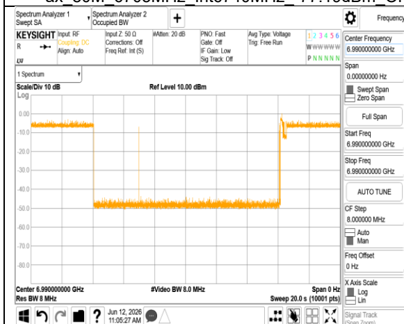
ax 80M_7025MHz_Int6990MHz_-76.07dBm Minimal
