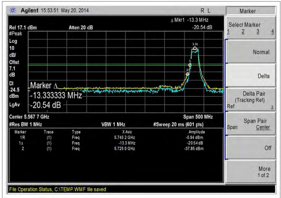
3dbi dual ants_11n-20_13.5dbm_5745MHz
