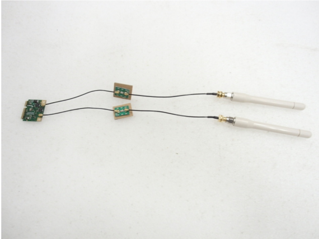
module with antenna (total cable length 0.15m)
