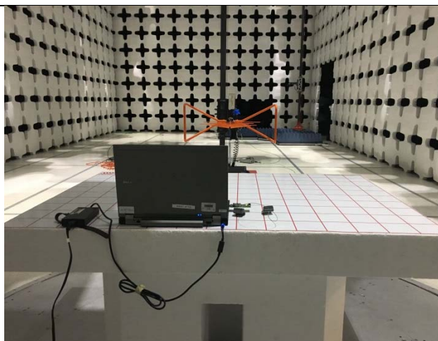
Radiated Emission Below 1G – Rear View
