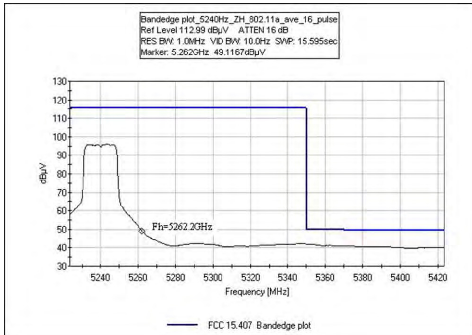
Band edge plot_5240Hz_ZH_802.11a_ave_16_pulse_orig
