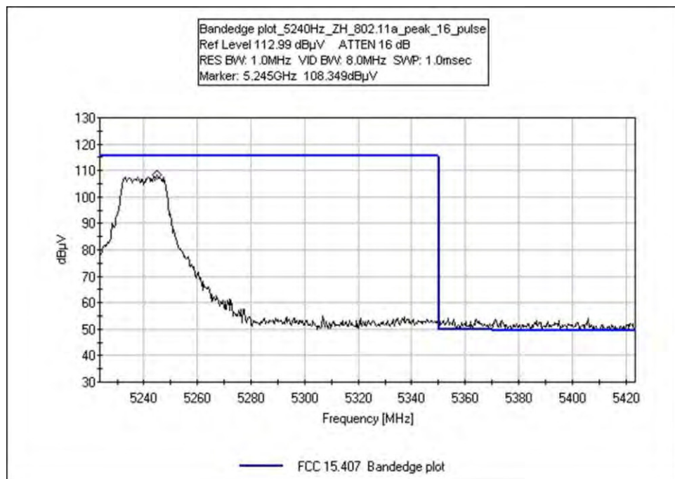
Band edge plot_5240Hz_ZH_802.11a_peak_16_pulse_orig
