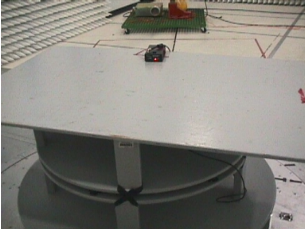
Conducted Emissions Test Configuration for Activator
