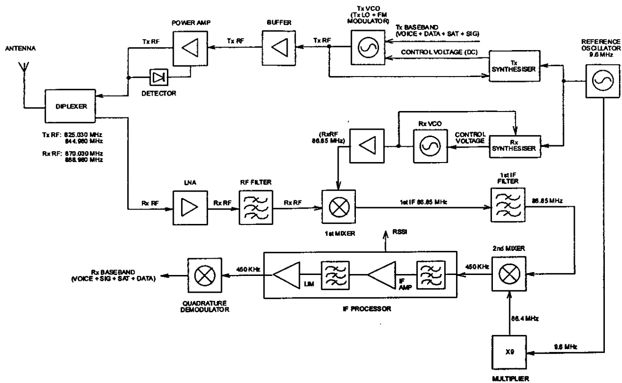
Figure 3-6 Block Diagram of RF
