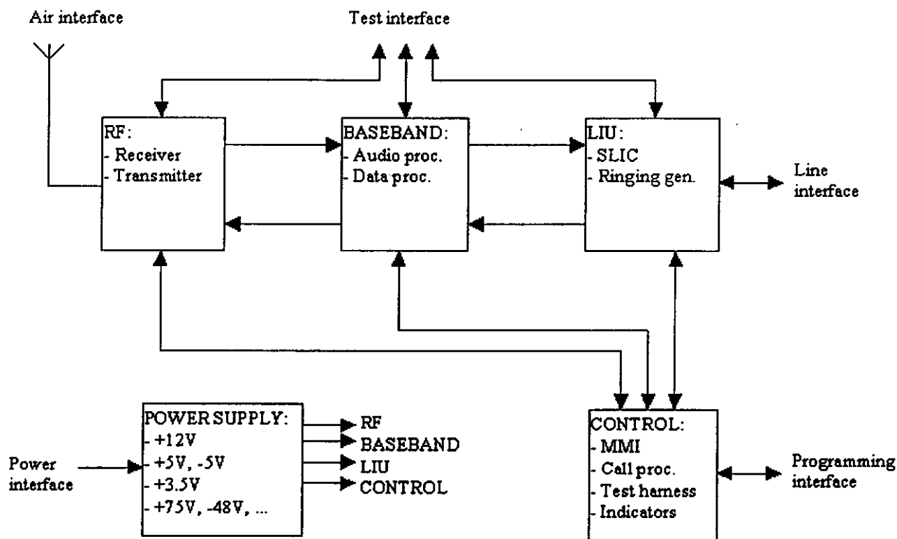
Figure 2-5 Block Diagram of SRT
