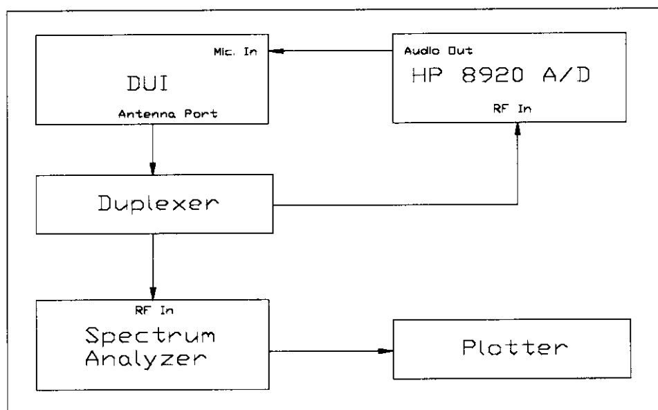
Set Up Figure 6 Spurious Emissions at Antenna Terminal Spurious Emissions measurement between 869 – 894 MHz.
