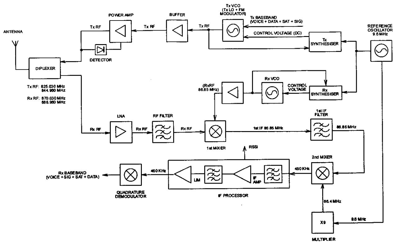
Figure 3-6 Block Diagram of RF U
