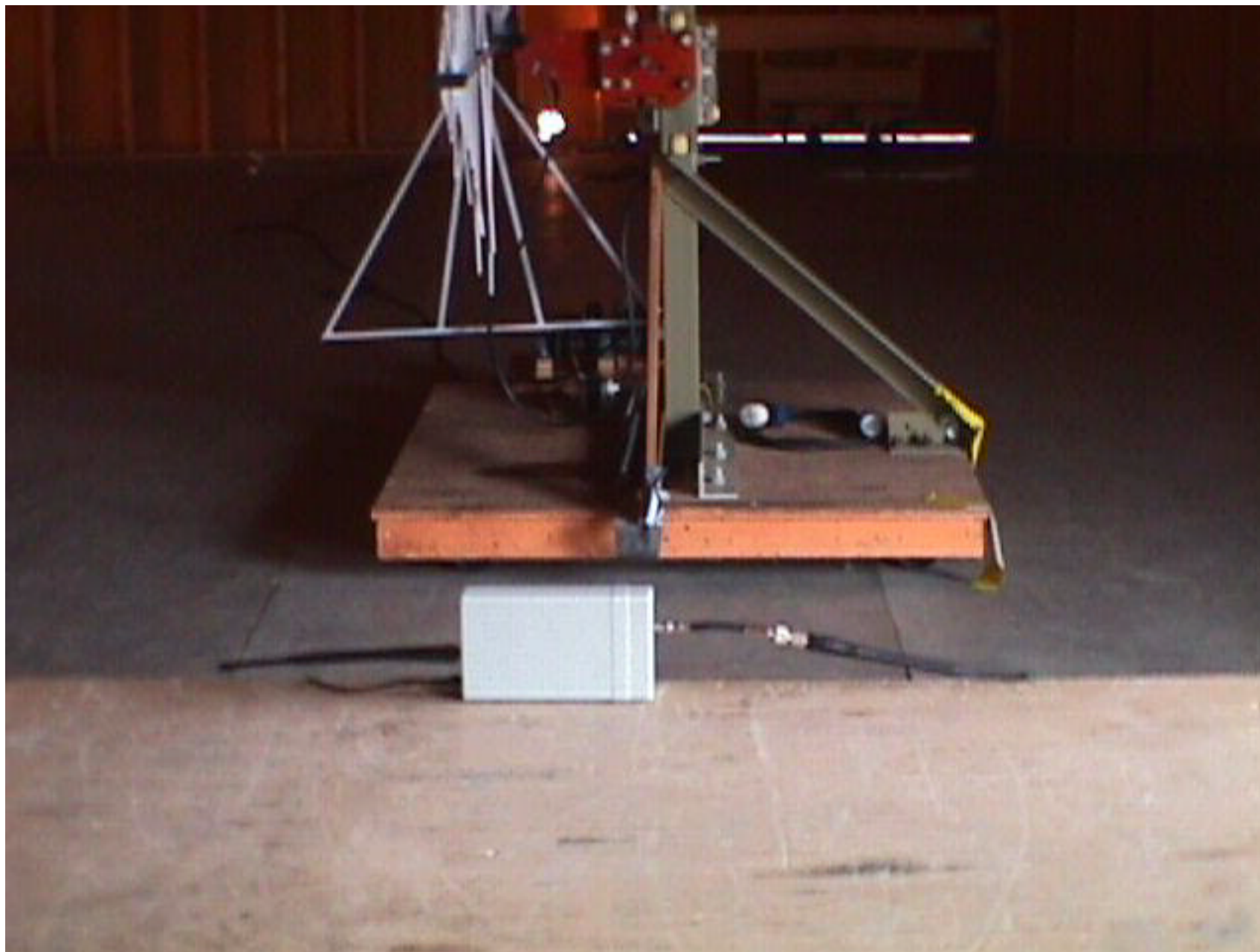
Radiated Emissions Test Setup Photograph # 1
