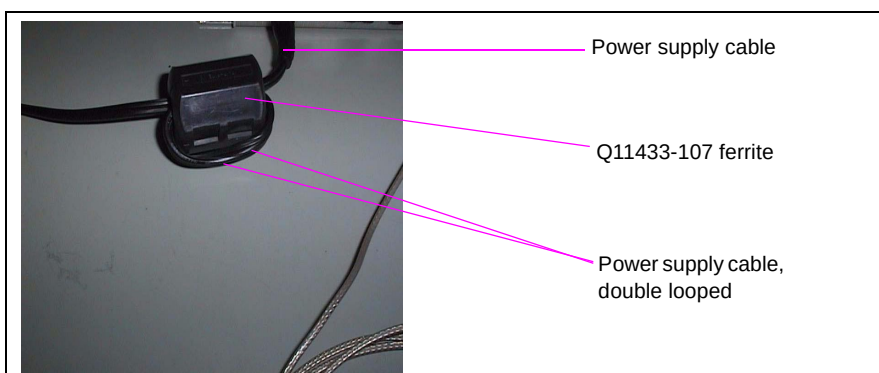
Figure: Power Supply (M01878B001) Cable with Ferrite
