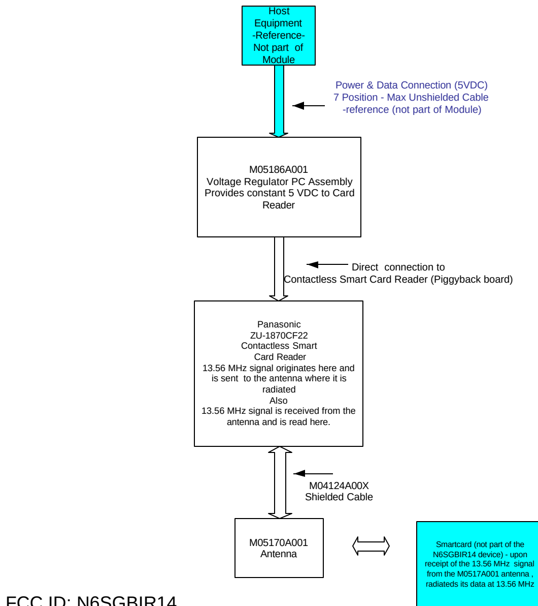
Figure 1: Block Diagram of the Contactless Smart Card Reader System
