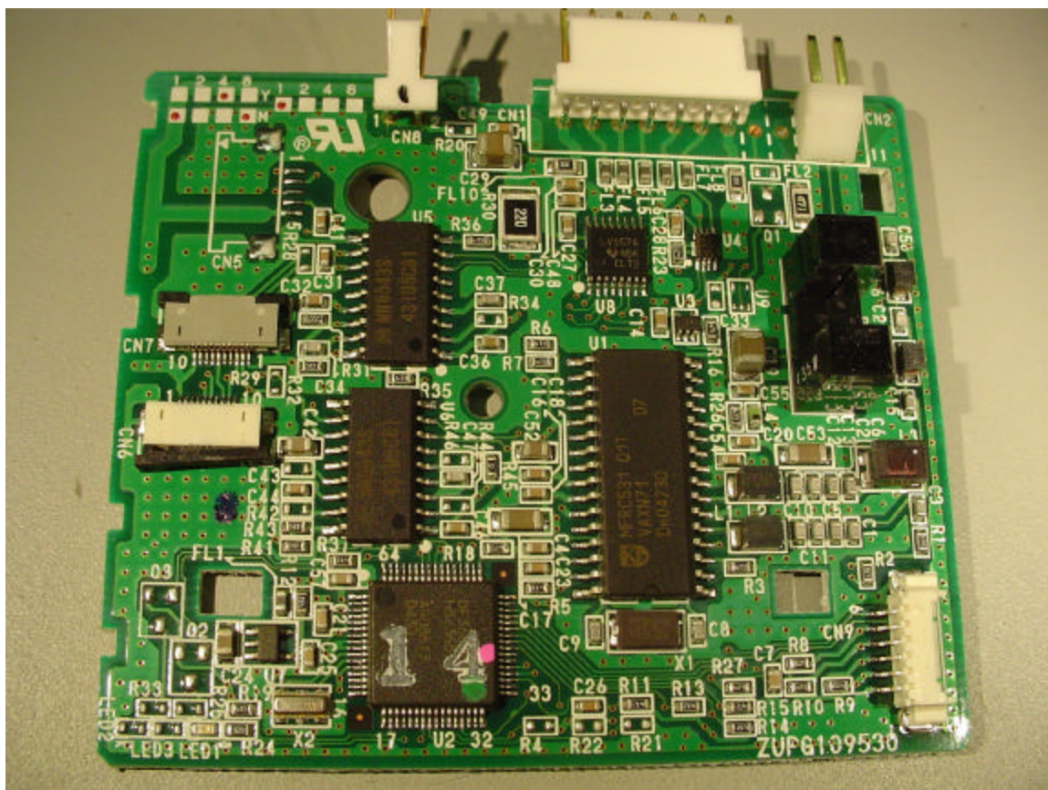
Internal View - Card Reader PCB, top view
