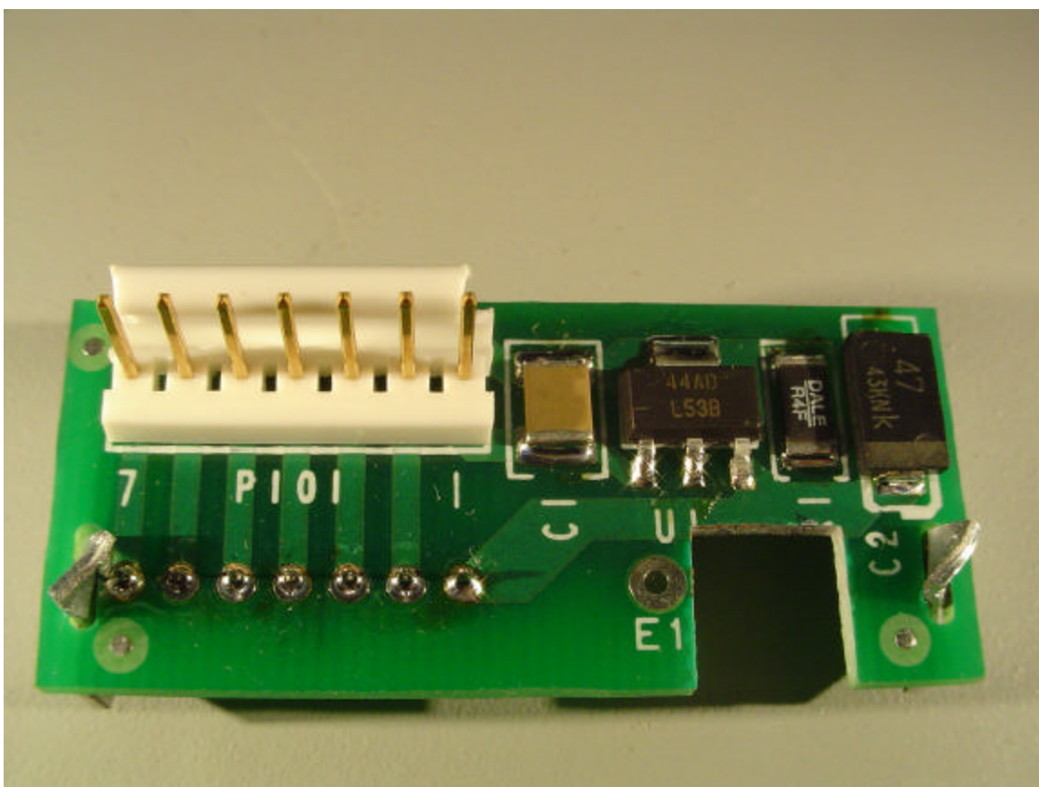
Internal View - M05186A001 Voltage Regulator PC Assembly, top view
