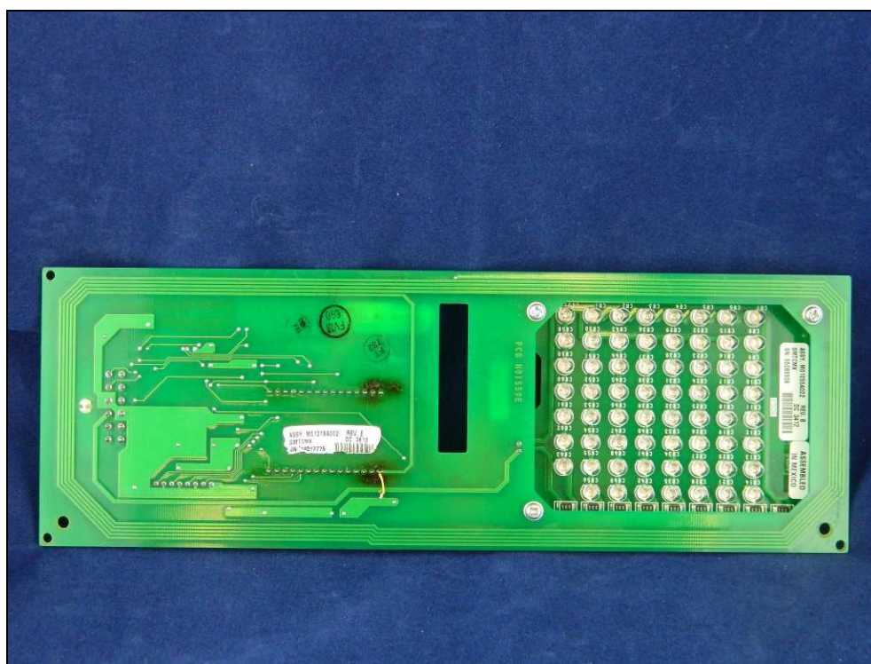
Figure 5: External/Internal Photograph
