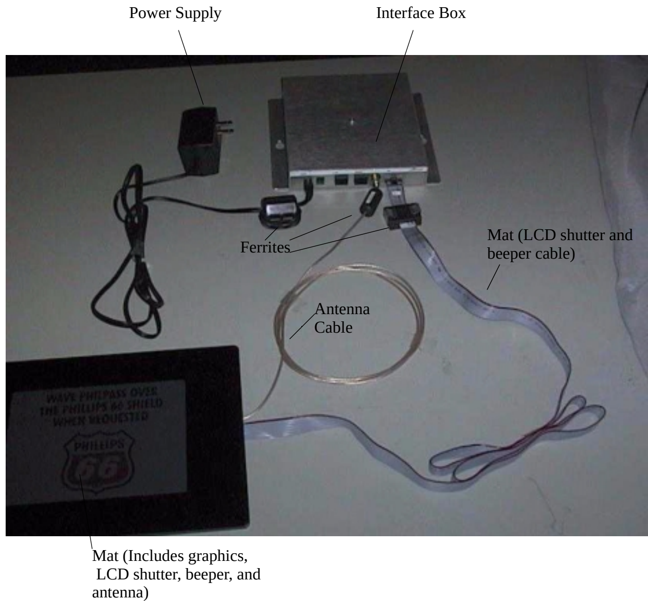
N6SMRIR12 Mat Reader 13.56 MHz - Overall Product View.
