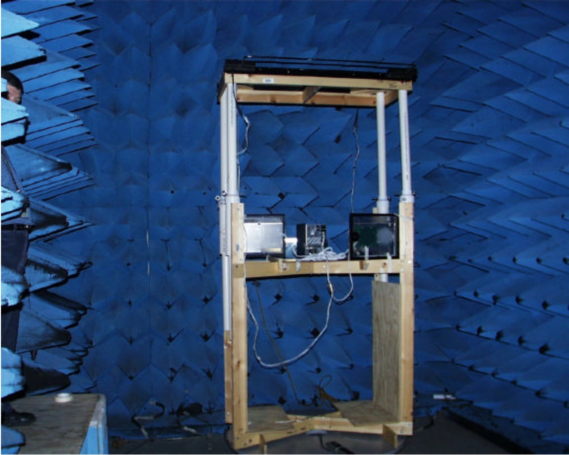
Radiated Emissions Pre-scan (Anechoic) Test Setup – Advantage Configuration
