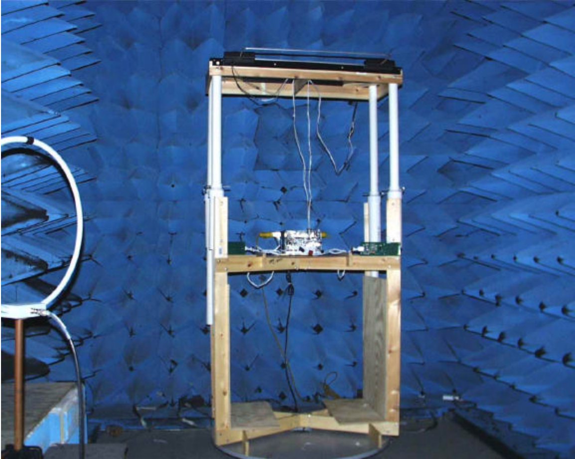
Radiated Emissions Pre-scan (Anechoic) Test Setup – Encore Configuration
