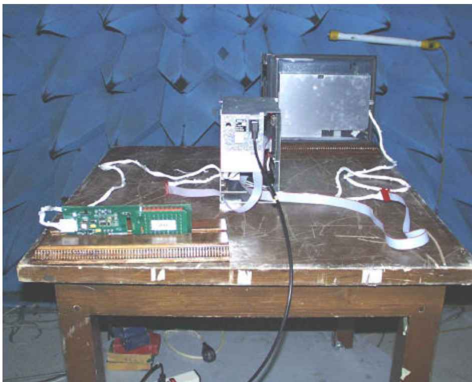
Radiated Emissions Pre-scan (Anechoic) Test Setup
