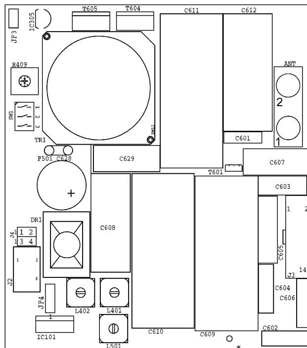
Figure 3: RFM Top View
