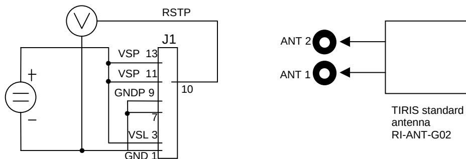
Figure 12: Noise Testing Configuration
