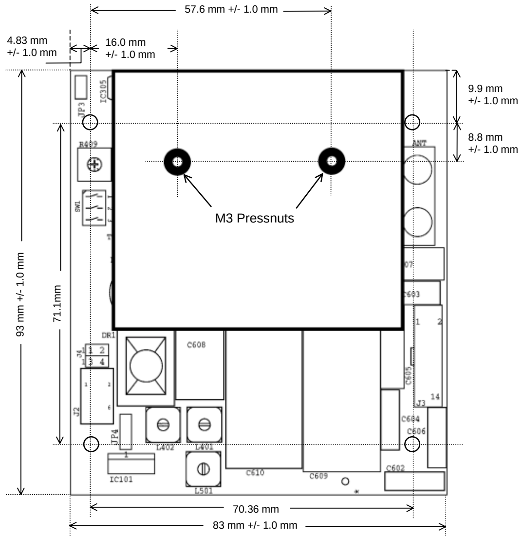
Figure 5: Mechanical Dimensions
