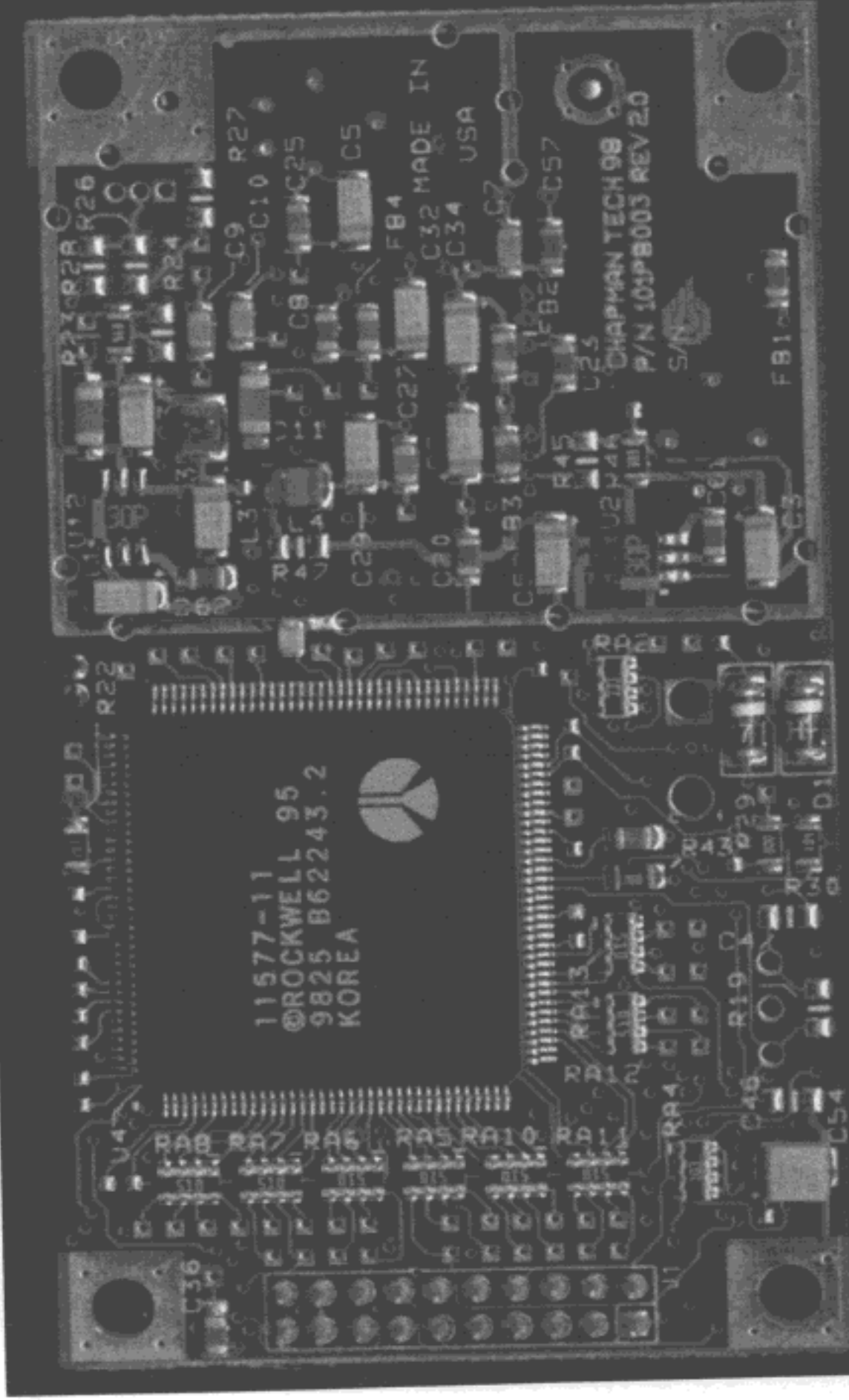
PHOTO #5 - GPS BOTTOM VIEW
