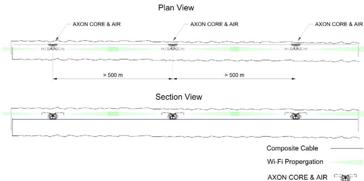
Figure 9: Installation scheme in a straight drive
