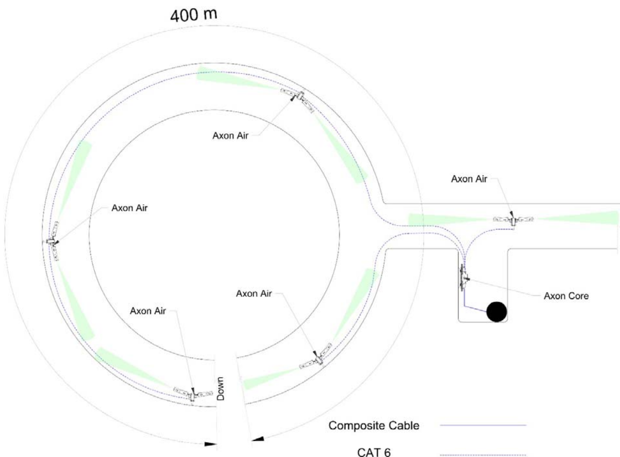
Figure 10: Installation scheme in a curved decline
