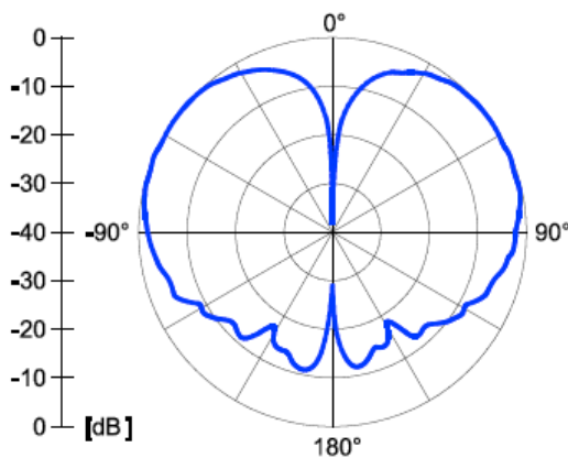
Vertical 5250 MHz
