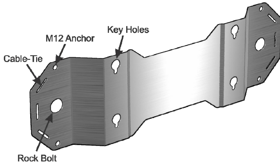
The AXON Core mounting plate
