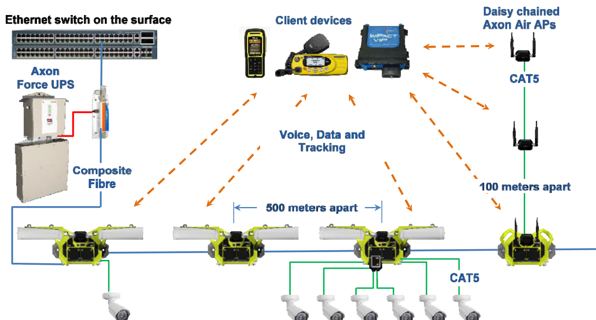
Figure 1: AXON system layout
