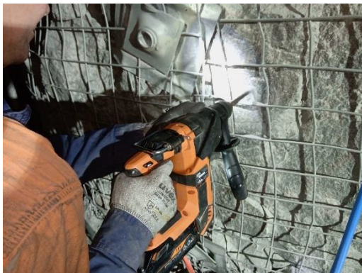
Step 1. Drill 13 mm hole
