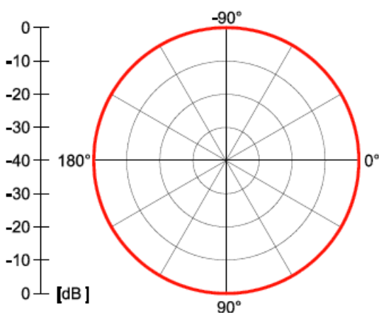
Horizontal 5250 MHz
