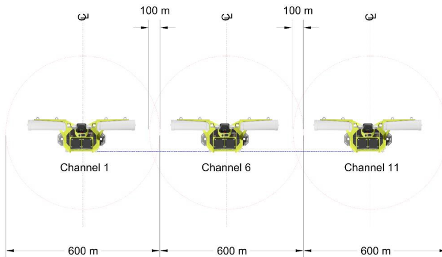
Figure 8: Wireless channel layout and distances around curves
