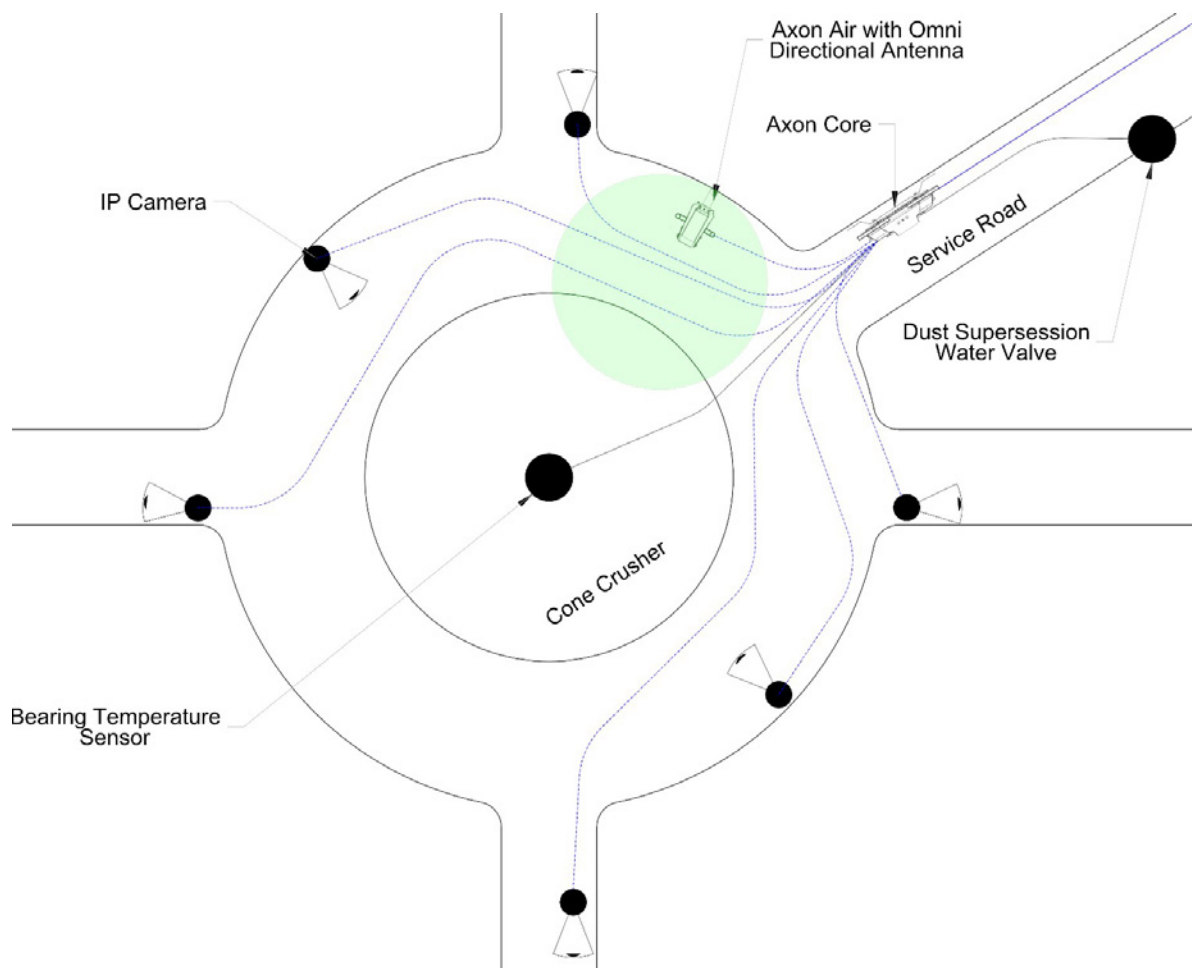
Figure 11: Installation scheme in a Crusher Building
