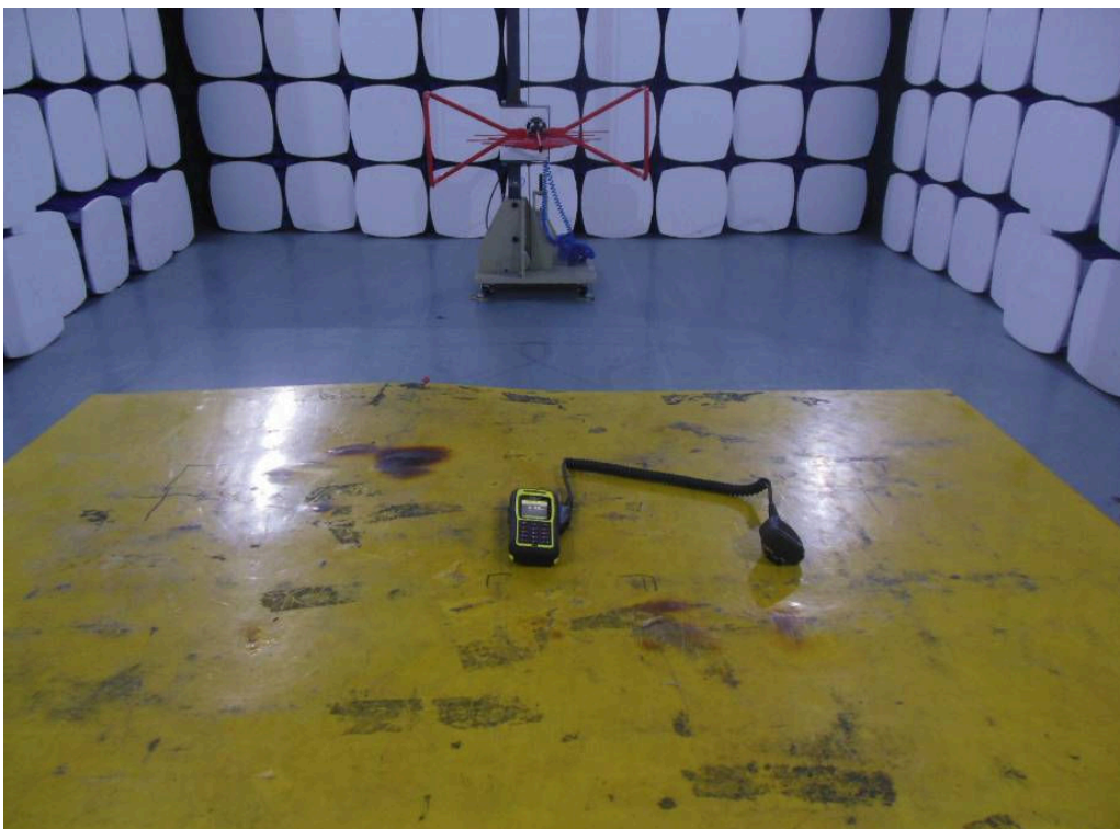
Radiated emission 30MHz~1GHz
