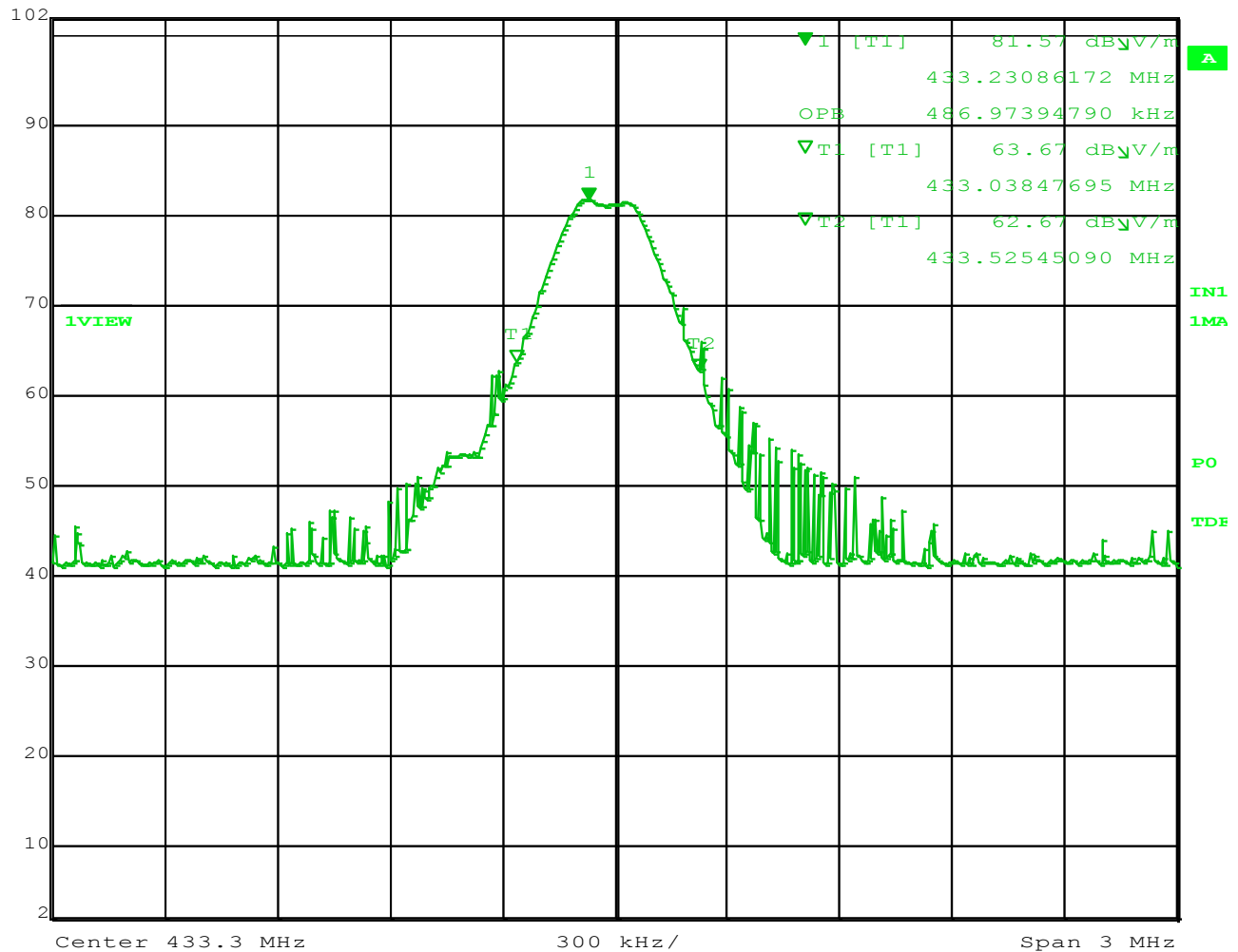
Figure 13 – 99% BW is 486.97 kHz
