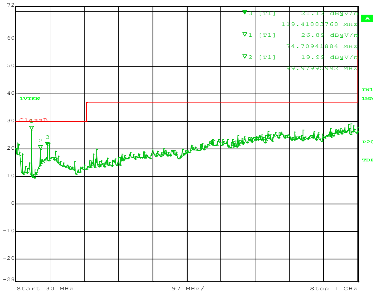
Figure 4 – Vertical 30 – 1000 MHz
