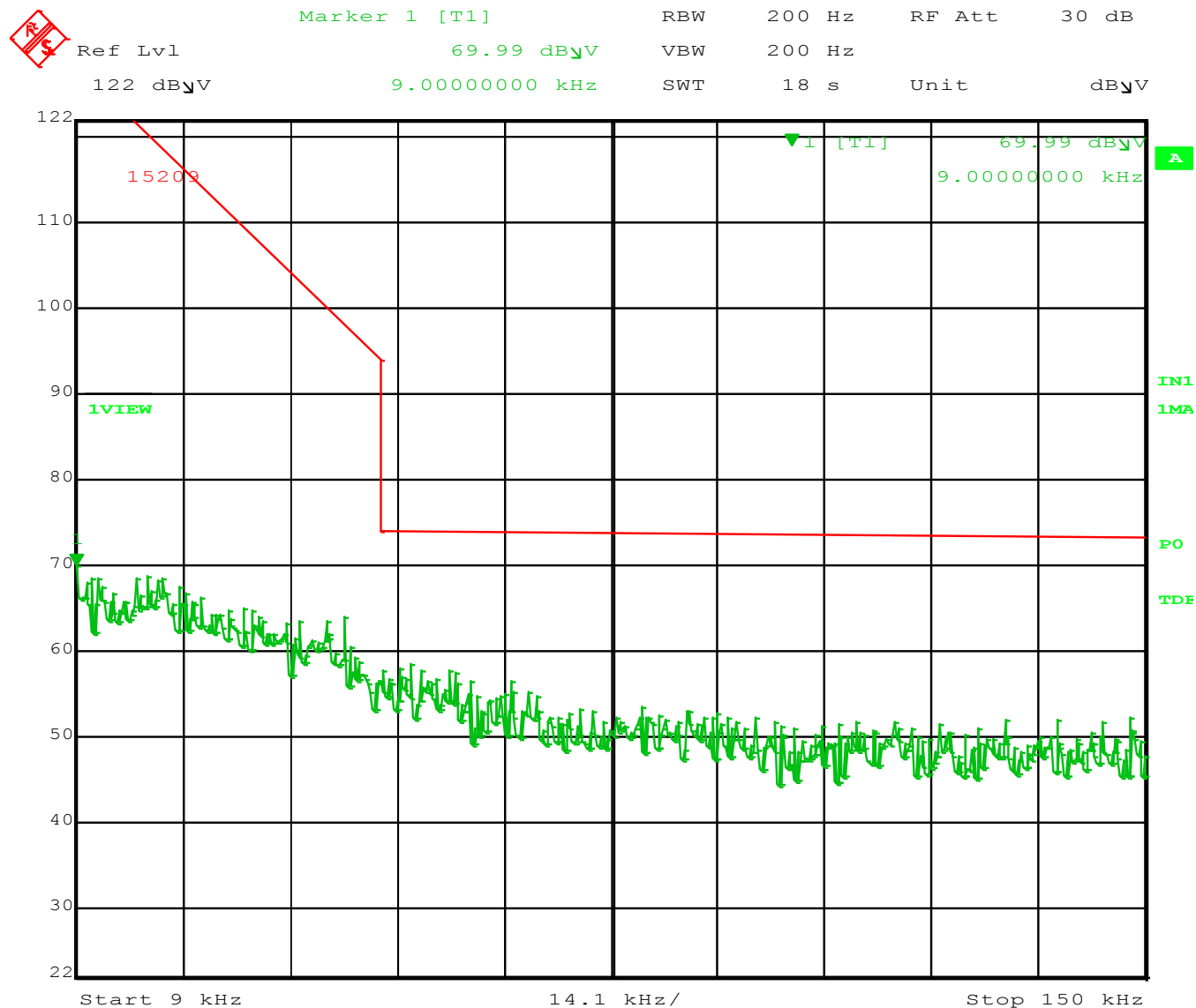
Figure 7 – Spurious Emissions (Perpendicular) 9 kHz to 150 kHz
