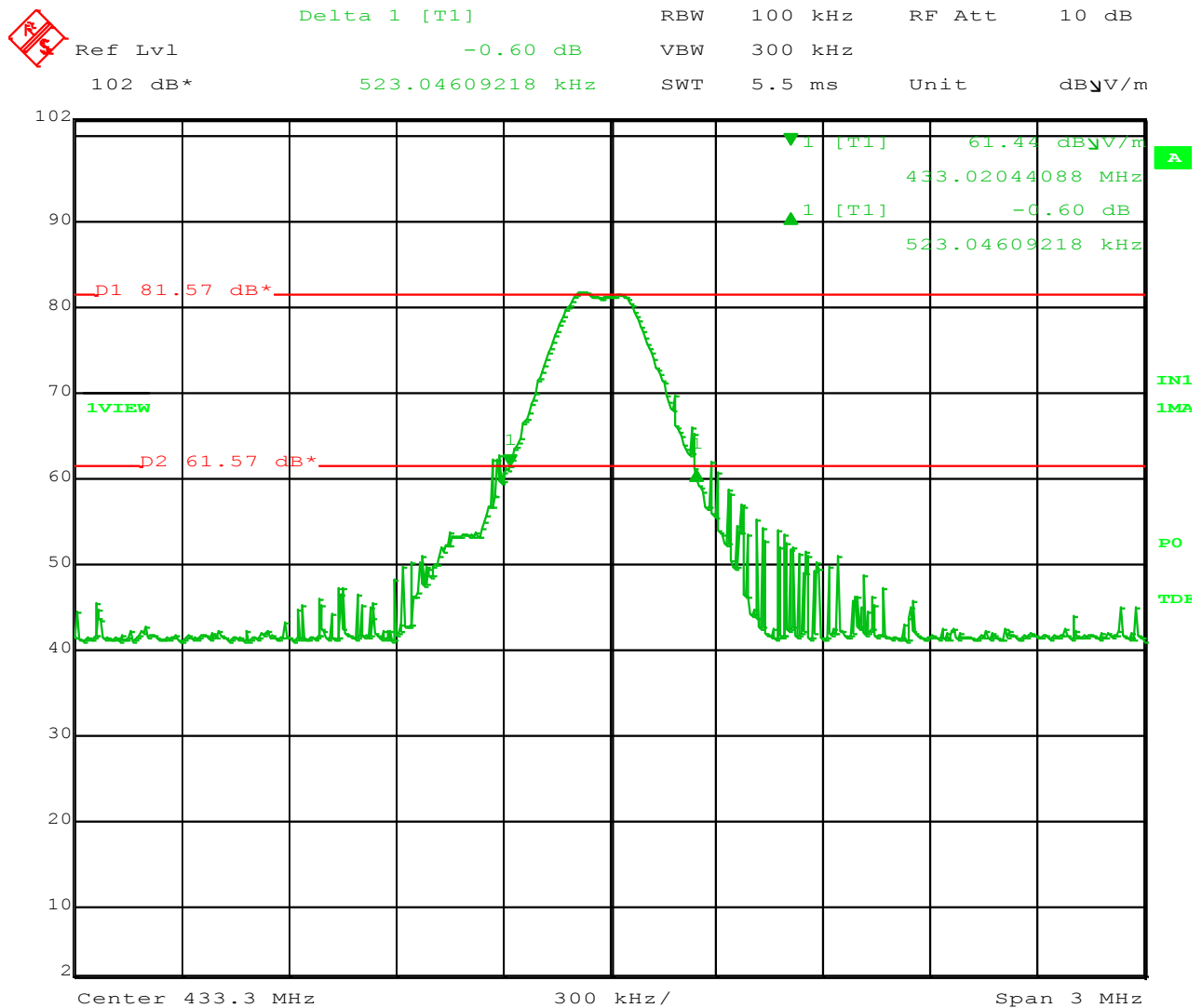
Figure 12 – 20 dB Bandwidth is 523.04 kHz
