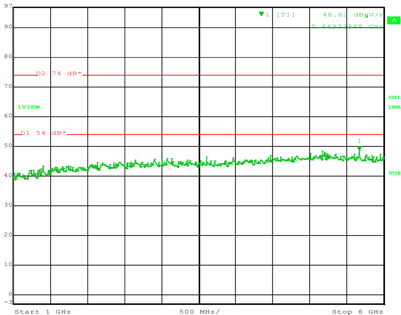
Figure 10 – Spurious Emissions (Horizontal) 1 to 6 GHz
