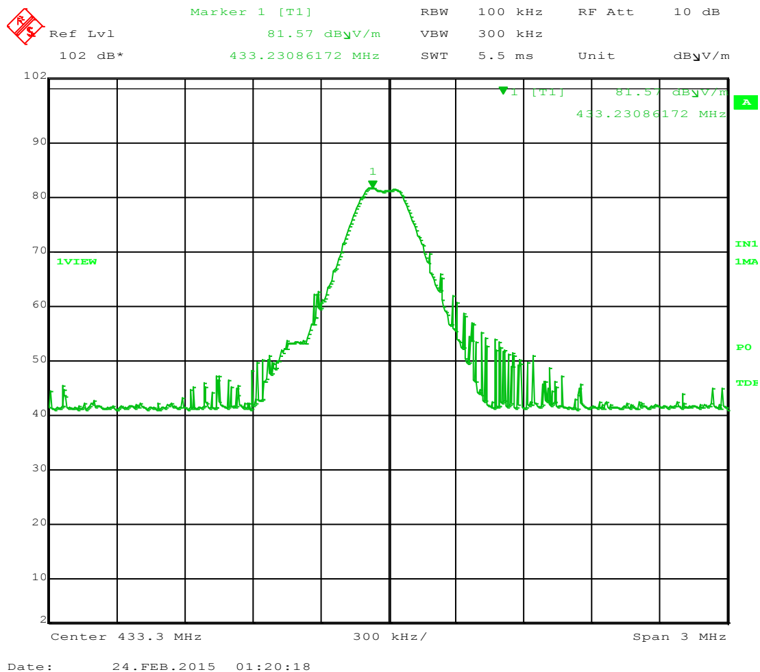
Figure 5 – Peak Field Strength Horizontal Polarity is 81.57 dBuV
