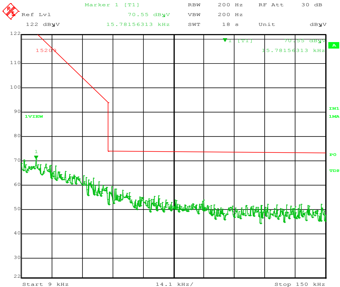
Figure 6 – Spurious Emissions (Parallel) 9 kHz to 150 kHz
