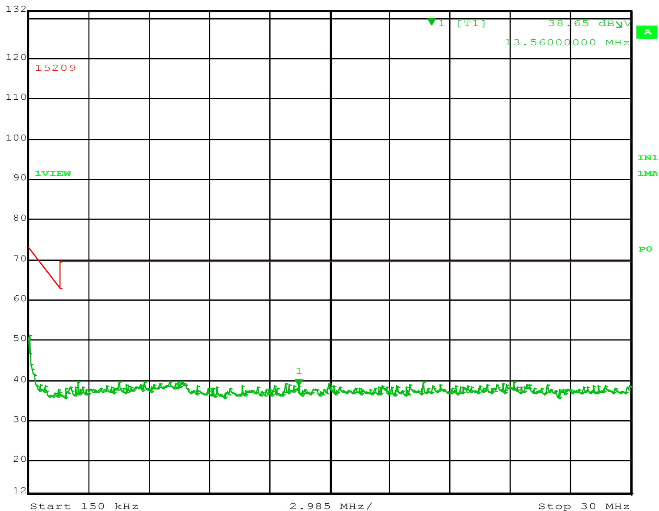
Figure 8 – Spurious Emissions (Parallel) 150 kHz to 30 MHz
