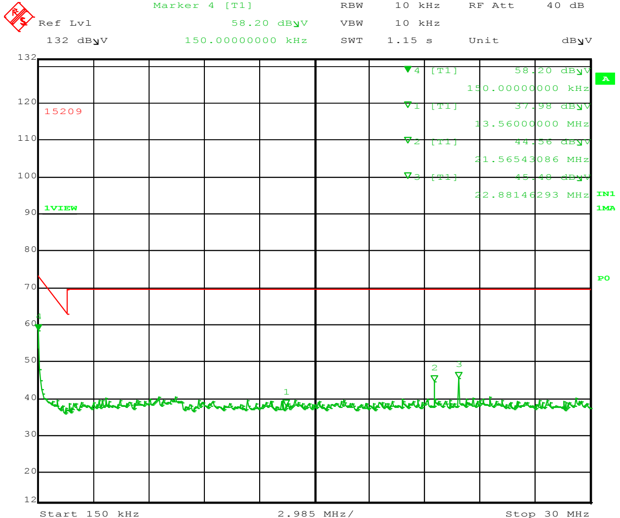
Figure 9 – Spurious Emissions (Perpendicular) 150 kHz to 30 MHz
