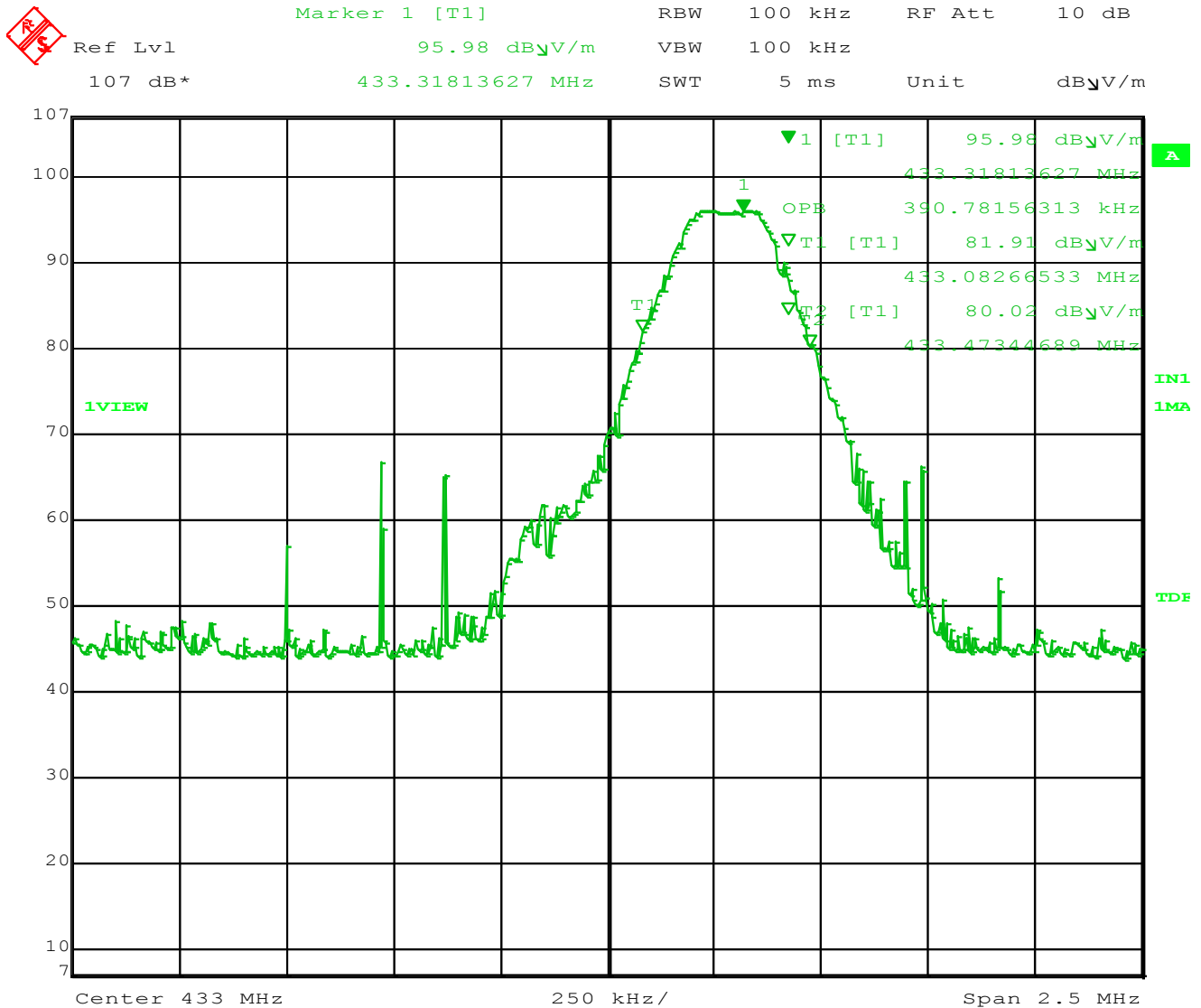
Figure 5 – 99% BW is 390.78 kHz
