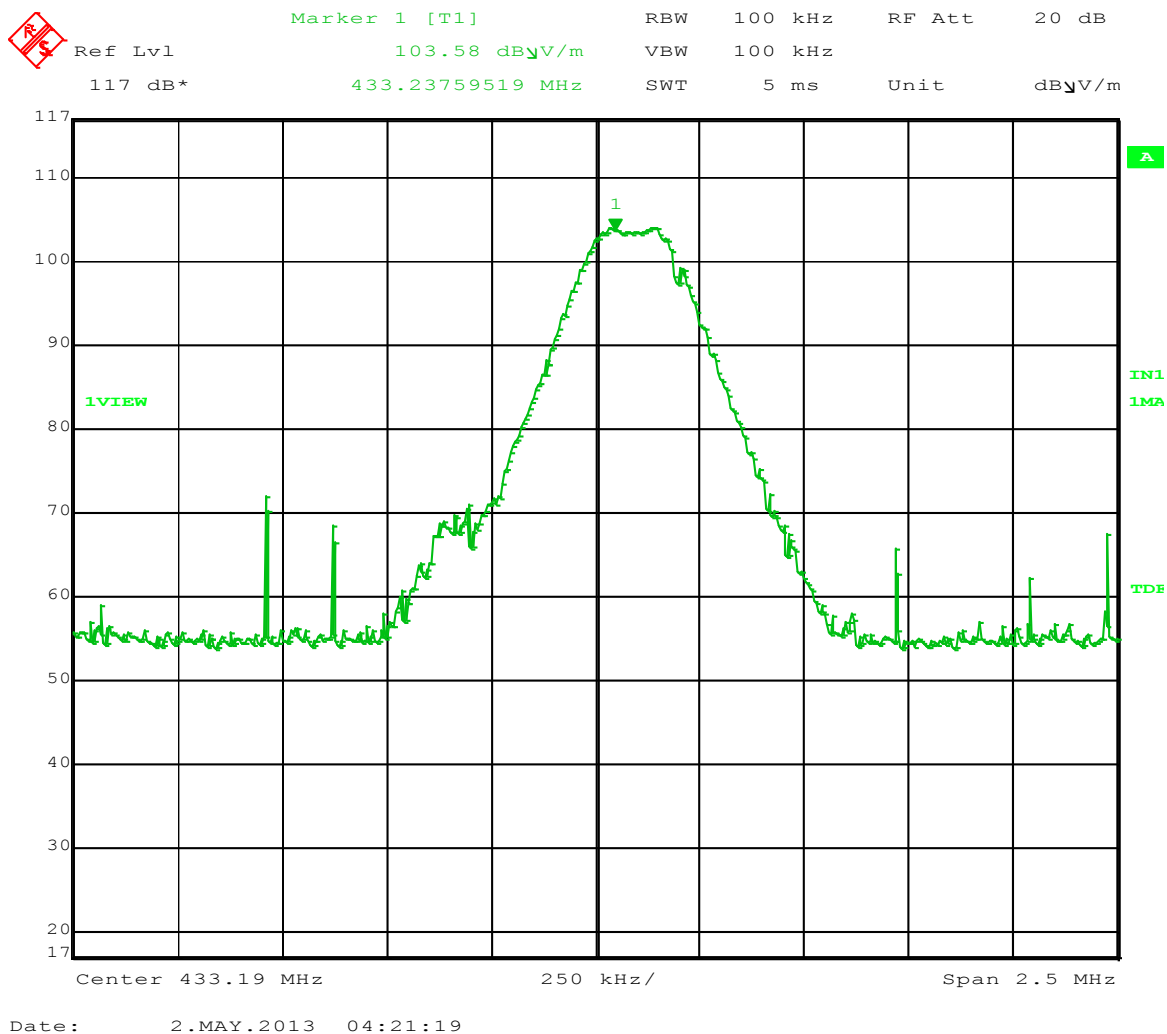
Figure 2 – Peak Field Strength is 103.58 dBuV at 3 meters, limit is 80.8 dBuV at 433 MHz
