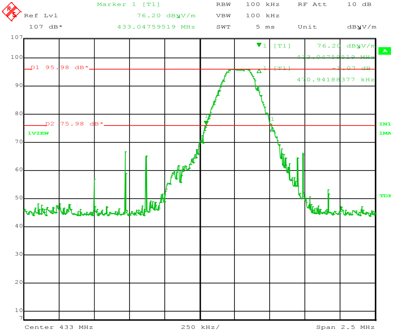
Figure 4 – 20 dB Bandwidth is 470.9 kHz
