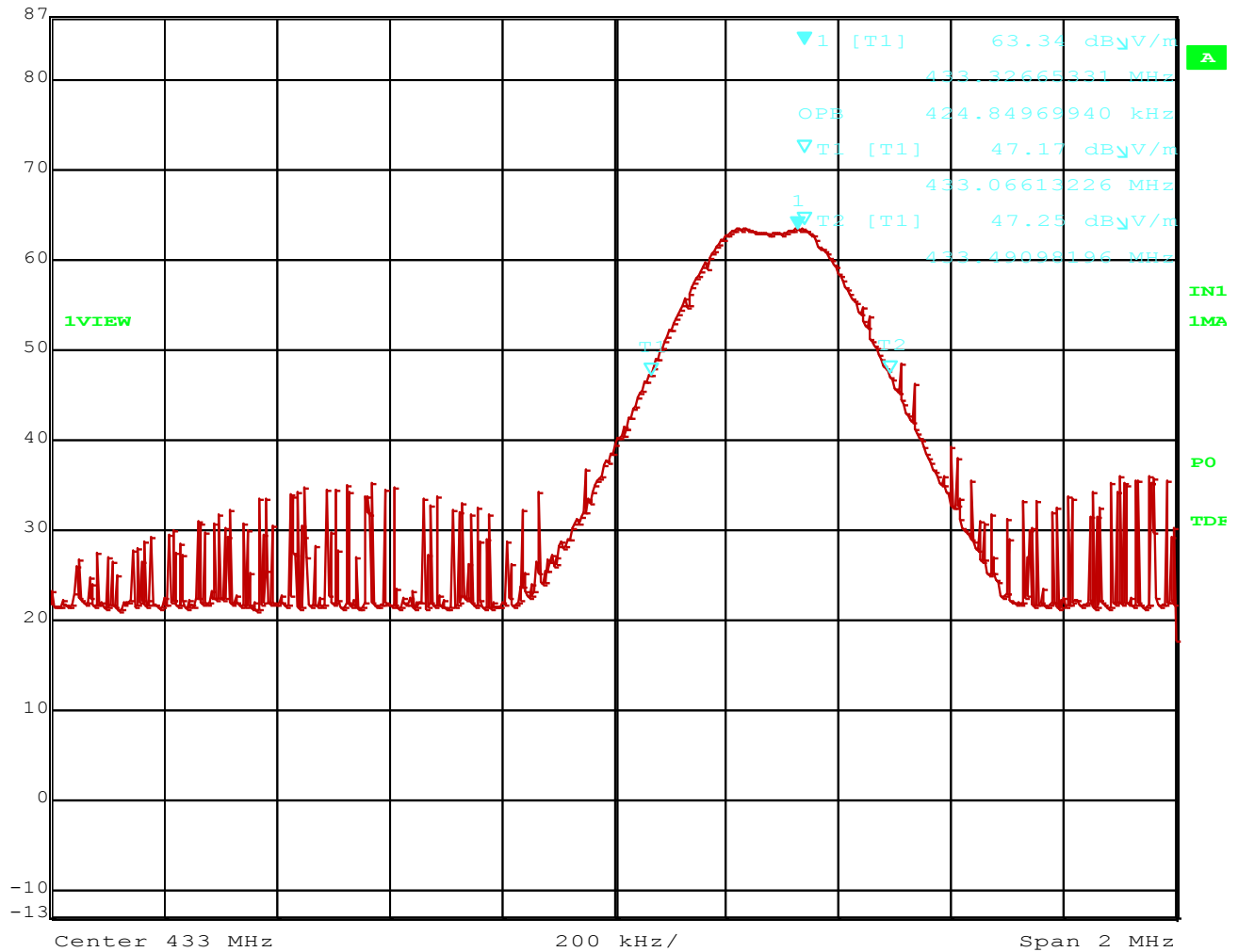
Figure 6 – 99% BW is 424.8 kHz
