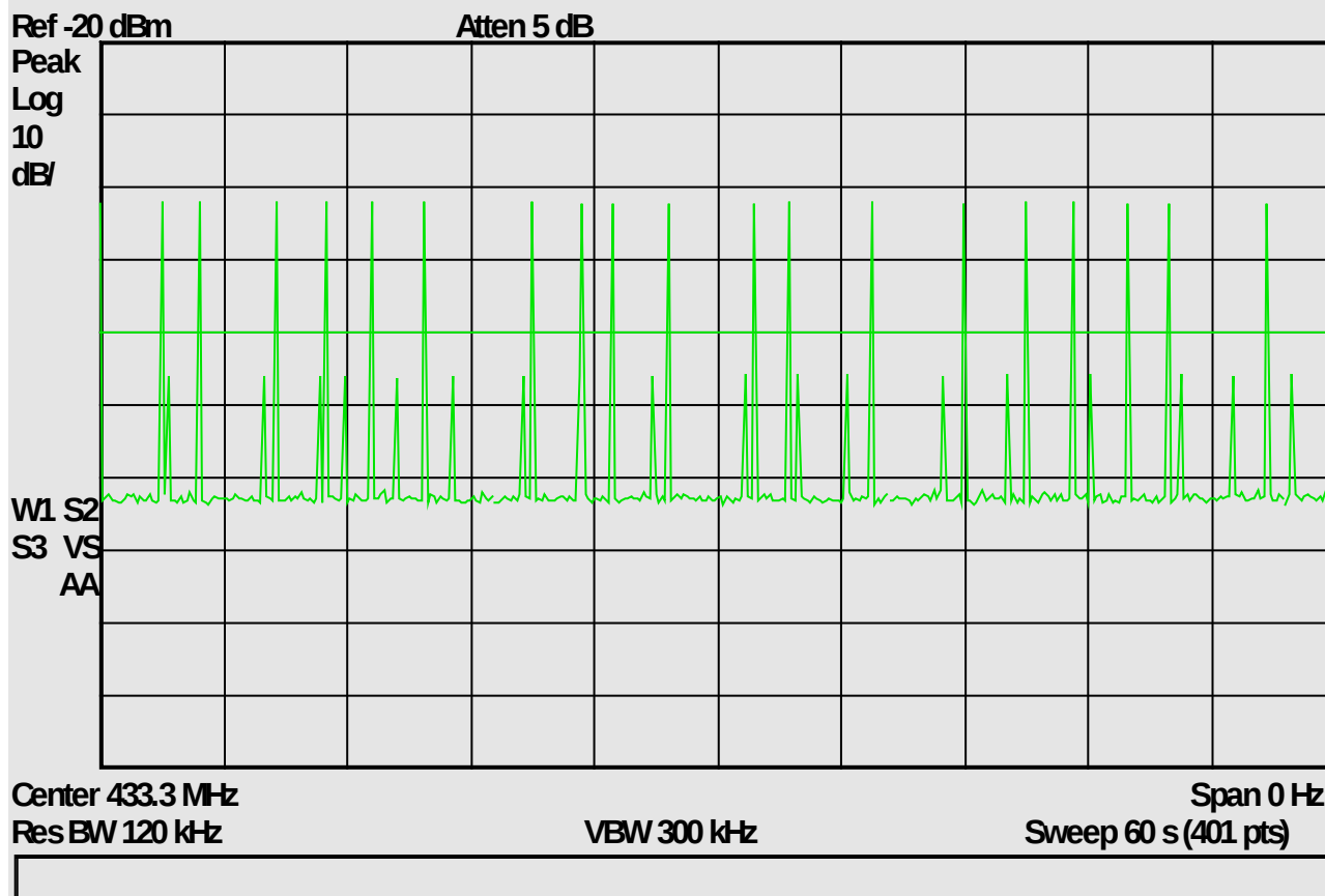
Figure 1 – 20 non-periodic pulses in 60 second
