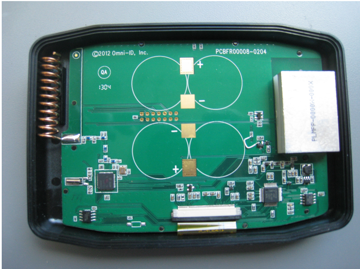
Component Side Internal Photograph
