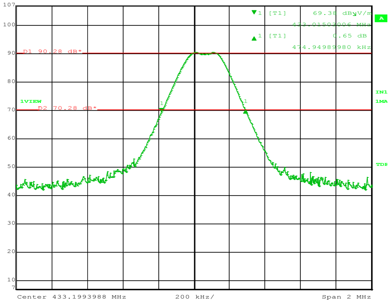
Figure 5 – 20 dB Bandwidth is 474.9 kHz
