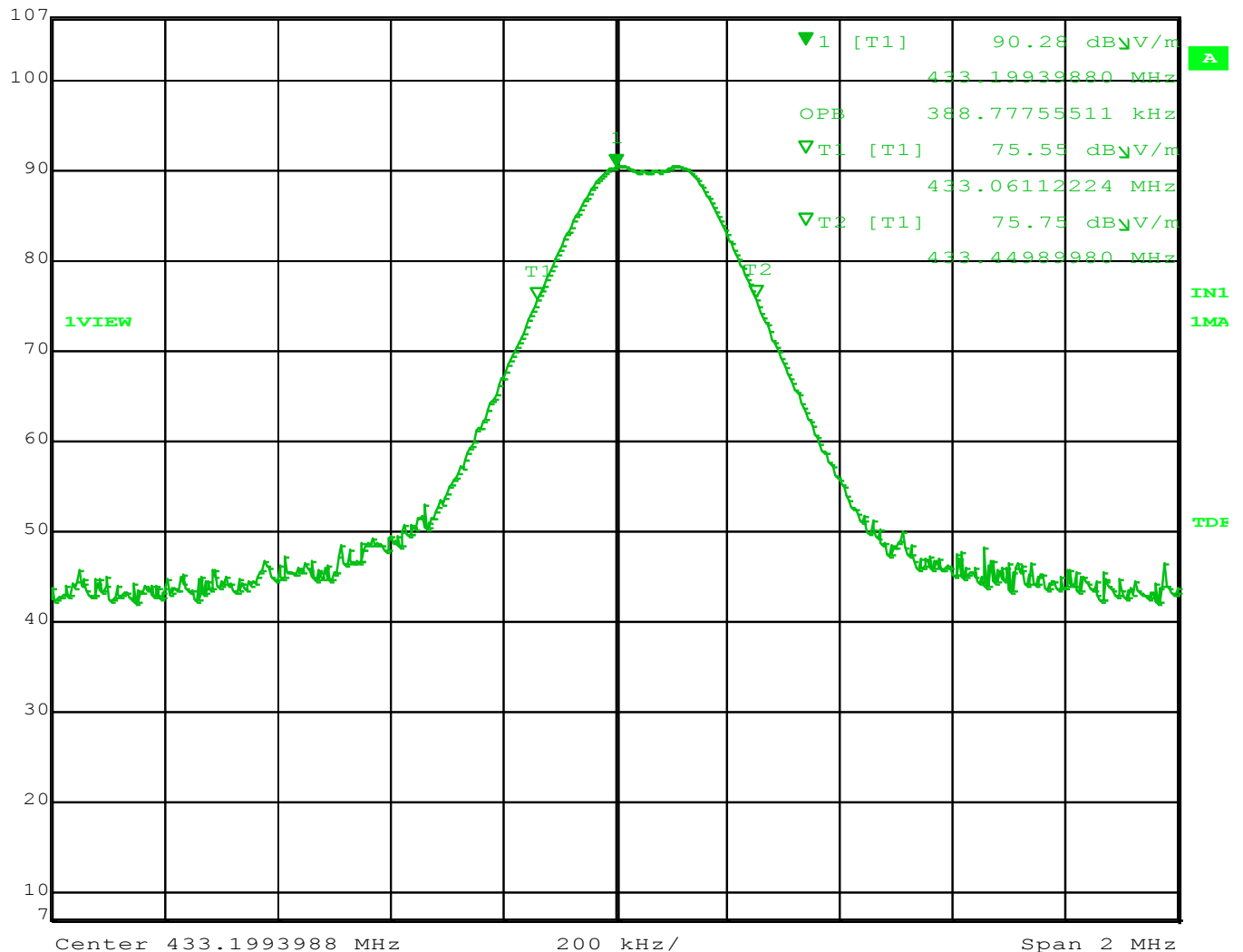
Figure 6 – 99% BW is 388.7 kHz
