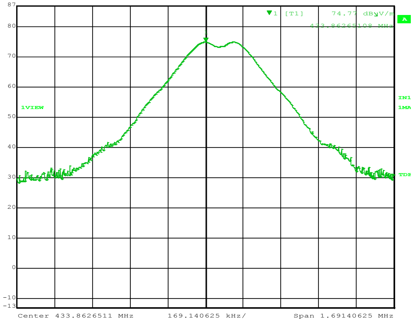
Figure 25 – Field Strength measurement with Yagi antenna
