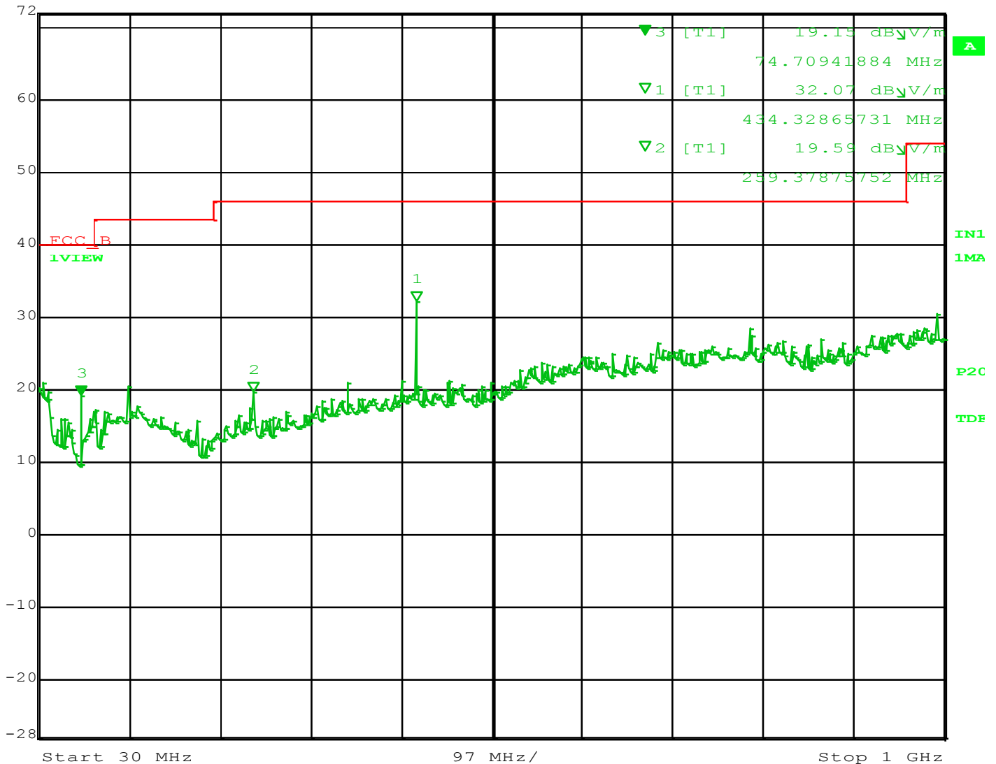
Figure 6 – Channel 13 with YAGI antenna, Vertical
