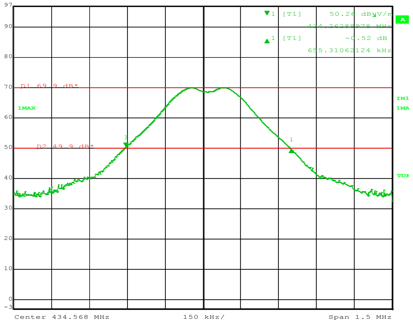
Figure 34 – 20 dB Bandwidth of channel 13 is 655.310 kHz
