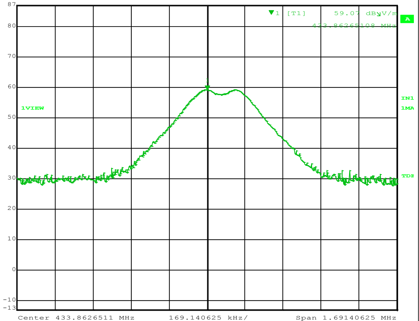
Figure 26 – Field Strength measurement with Yagi antenna
