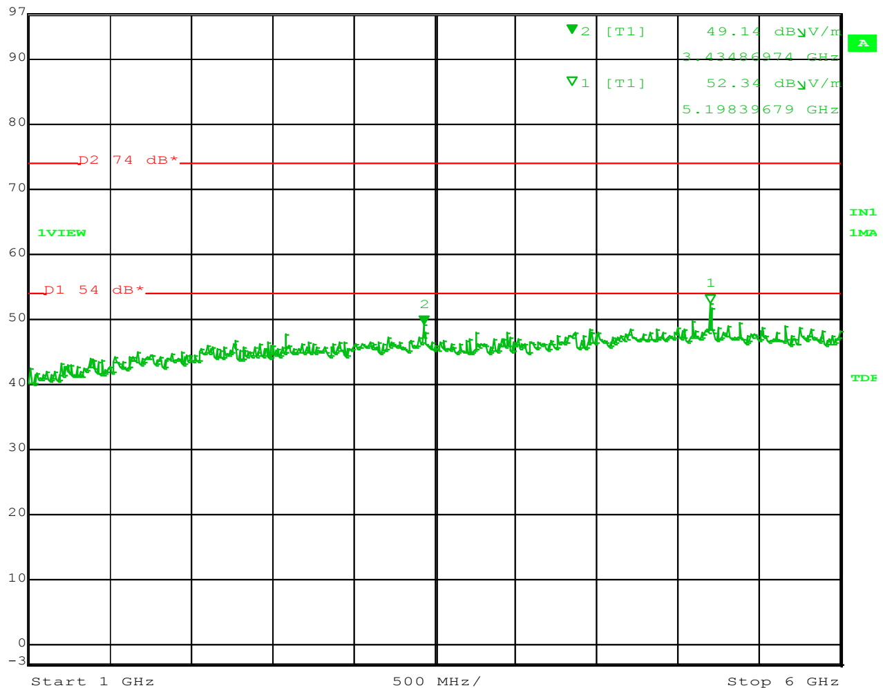
Figure 29 – Spurious Emissions (Horizontal) 1 to 6 GHz Channel 0
