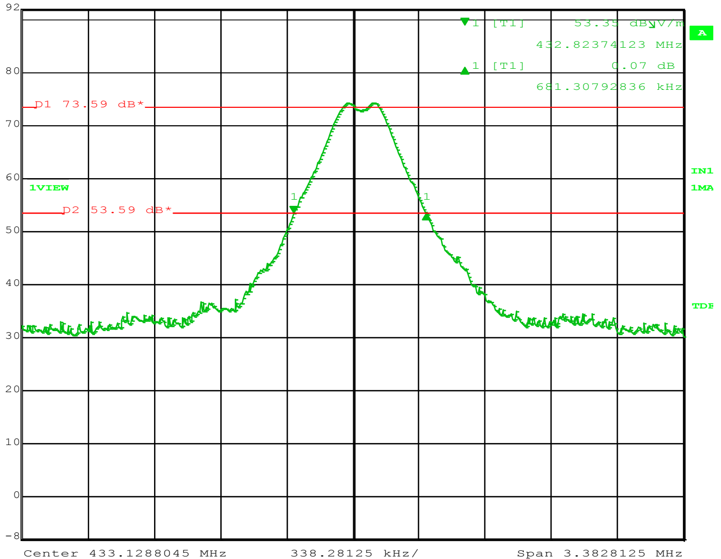
Figure 32 – 20 dB Bandwidth of channel 0 is 681.30 kHz
