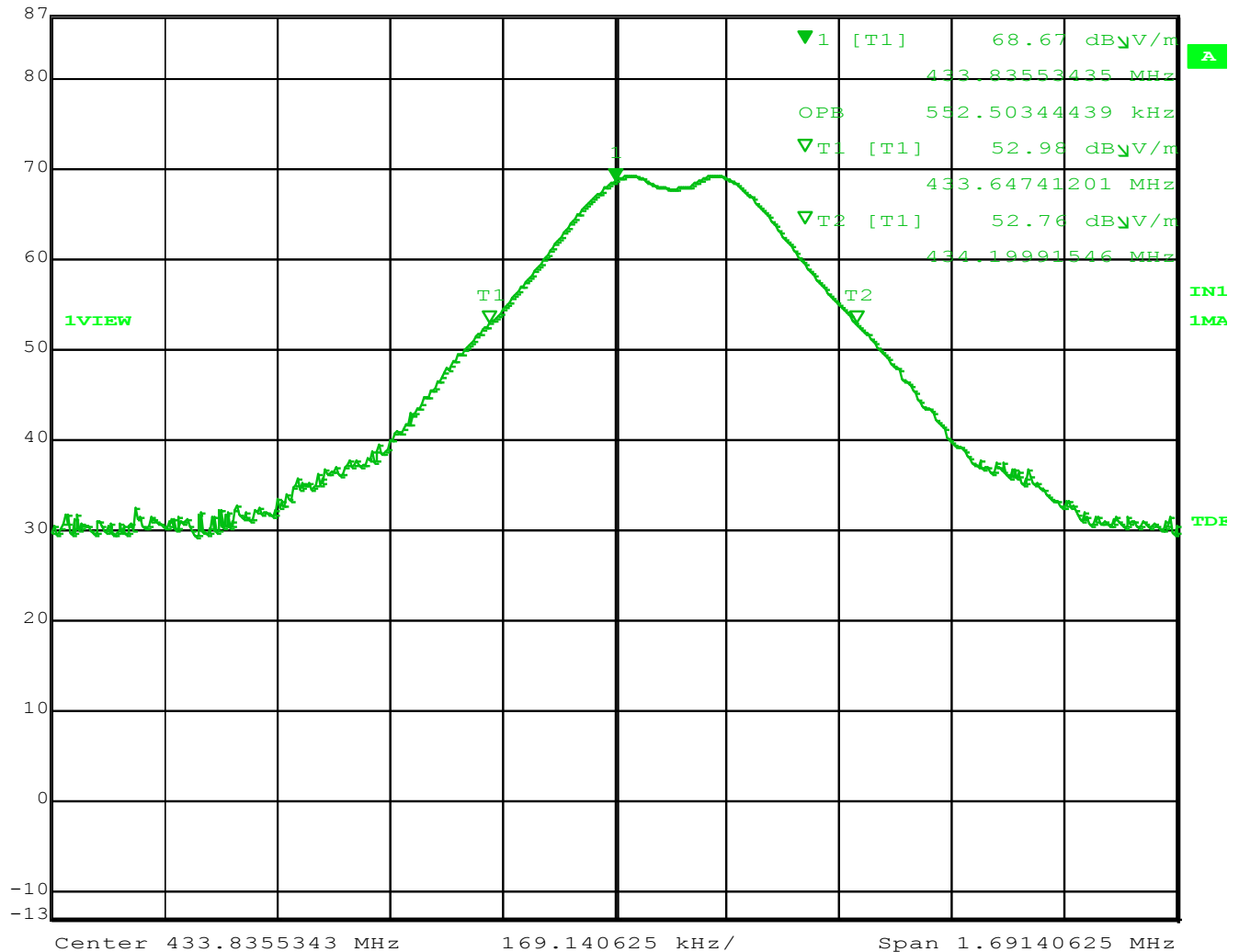
Figure 36 – 99% BW of channel 7 is 552.50 kHz
