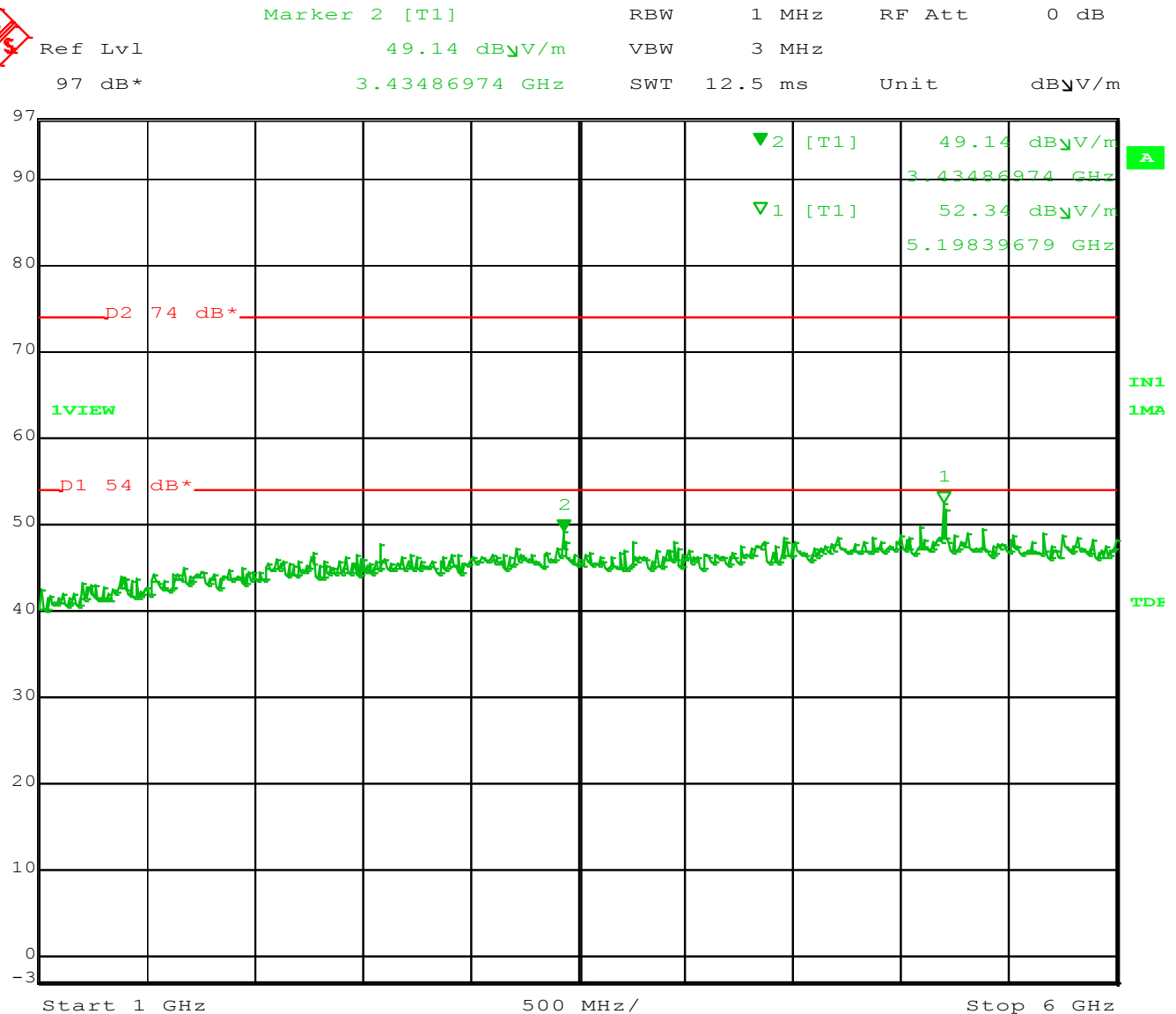
Figure 8 – Channel 0 Yagi Antenna, Horizontal
