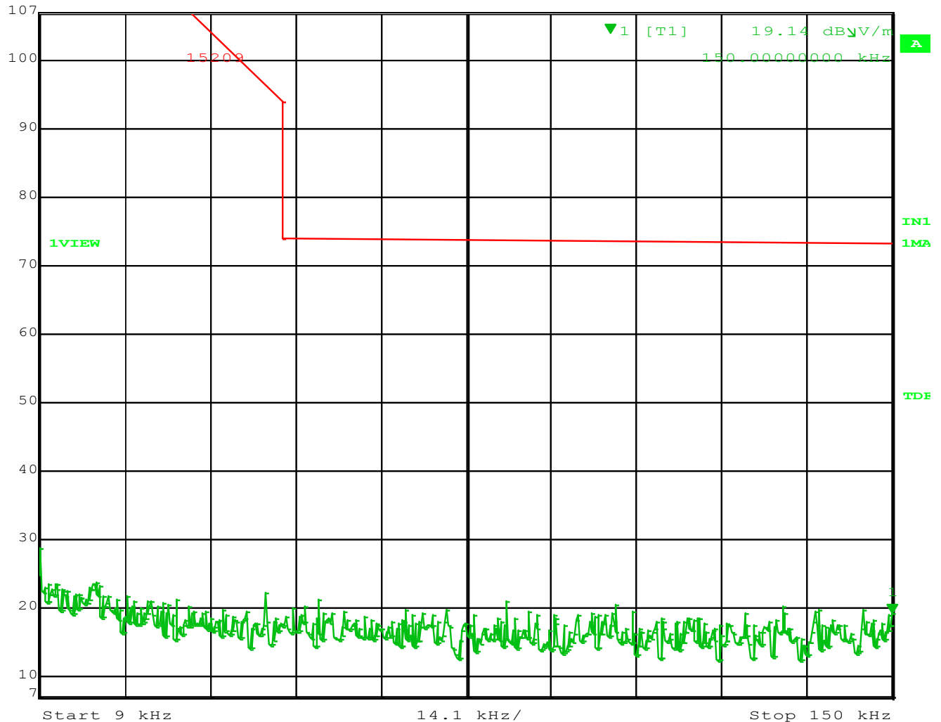
Figure 2 – Spurious Emissions (Perpendicular) 9 kHz to 150 kHz
