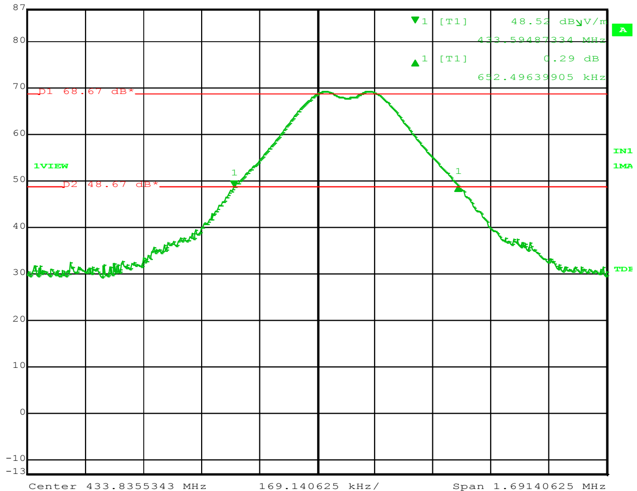
Figure 33 – 20 dB Bandwidth of channel 7 is 652.49 kHz
