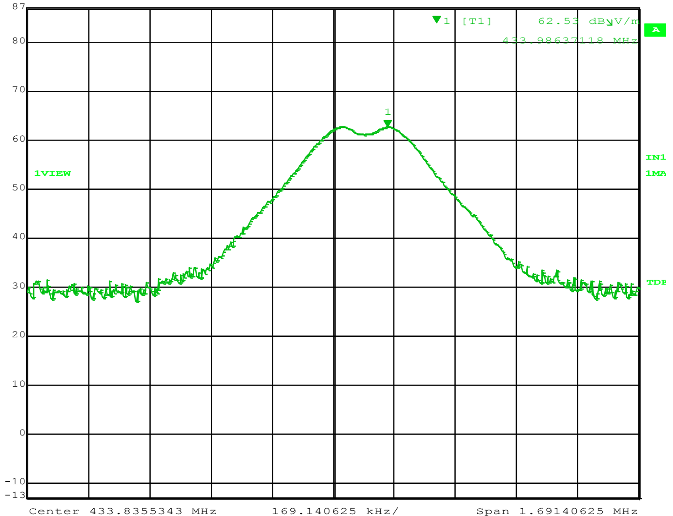
Figure 14 – Field Strength measurement with dipole antenna
