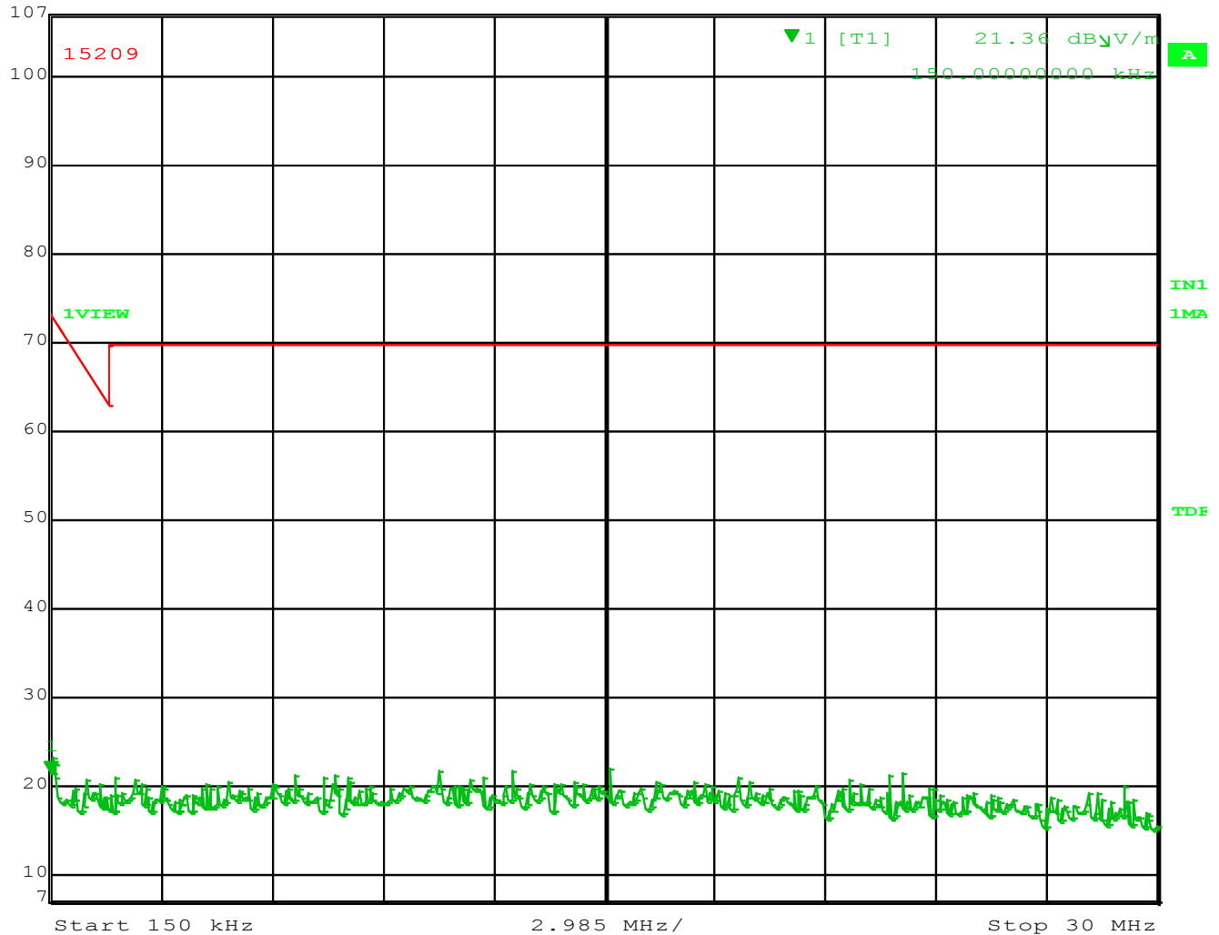
Figure 4 – Spurious Emissions (Perpendicular) 150 kHz to 30 MHz
