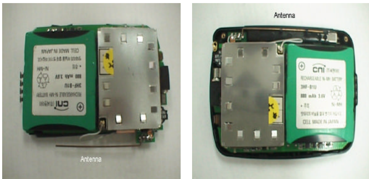
Figure 2: Antenna location
