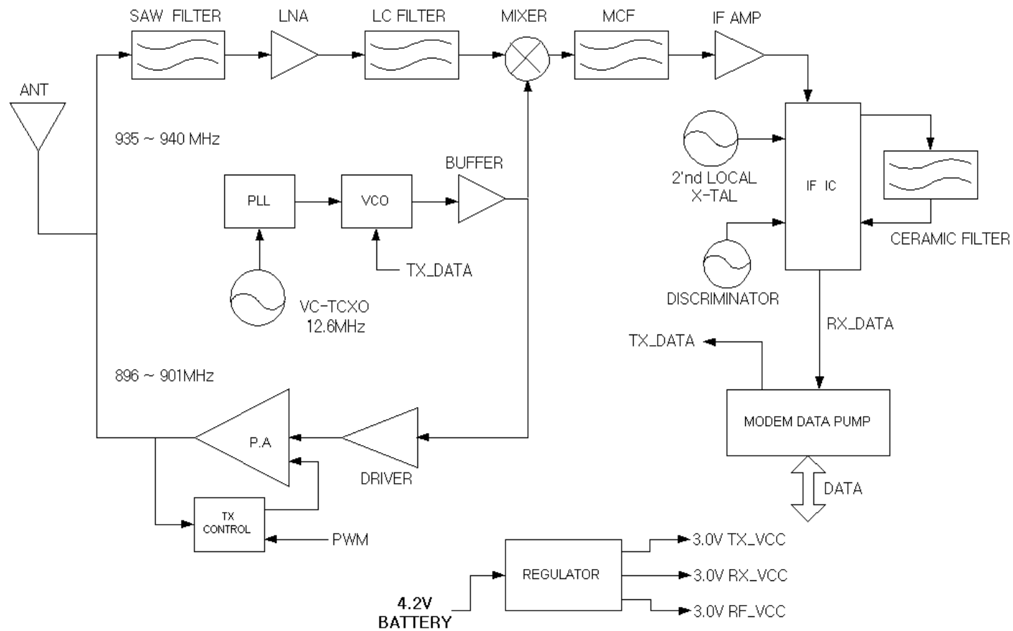
CNI-903M RF Block Diagram
