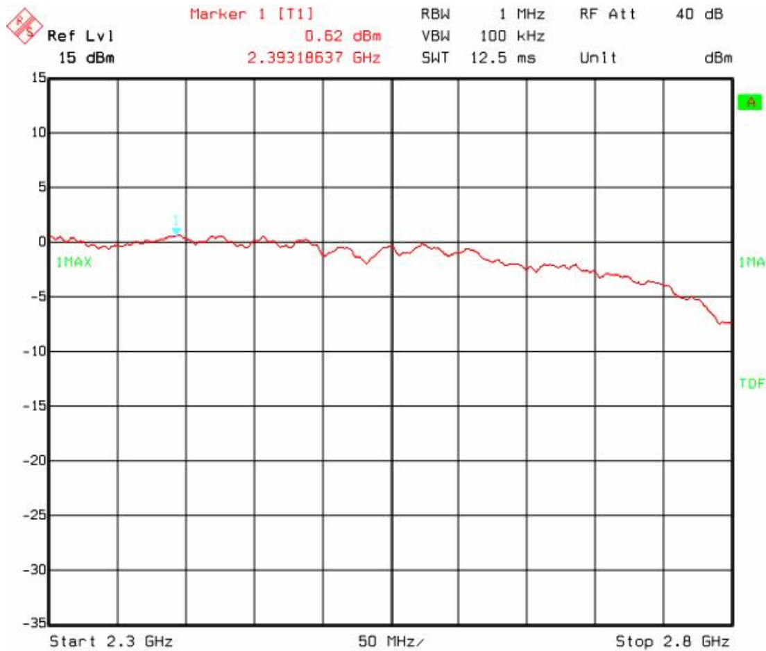
Figure 16: Output Power, PCBA in Laptop
