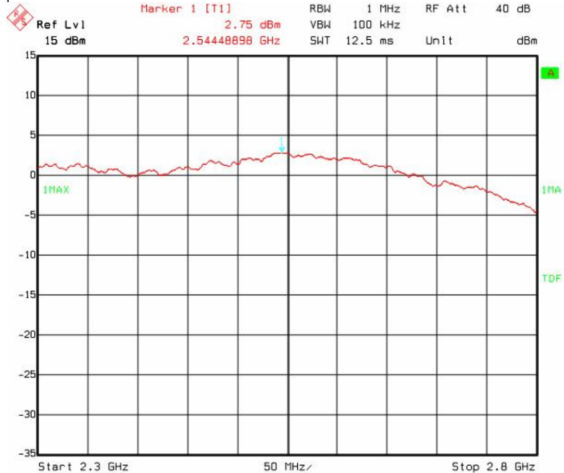
Figure 15: Output Power, PCBA
