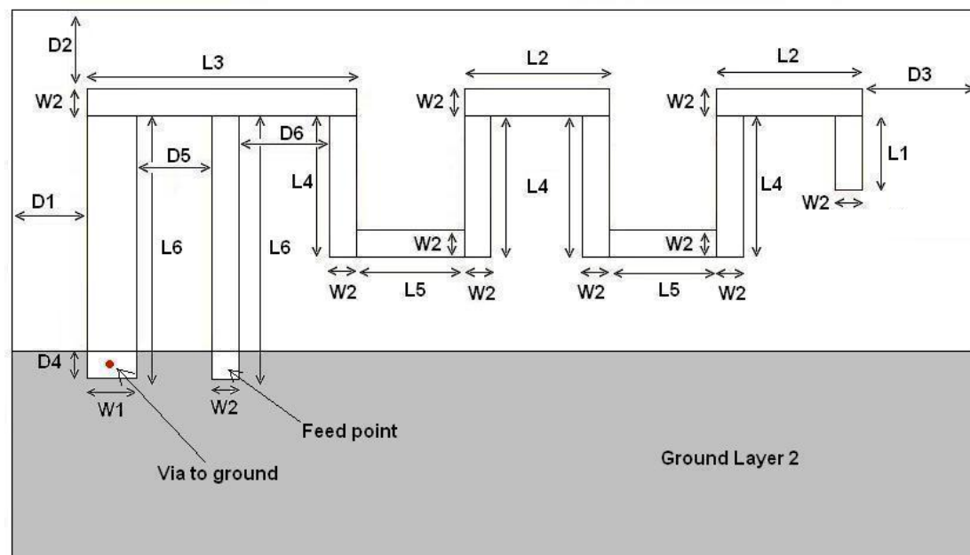
Figure 3: Antenna Dimensions
