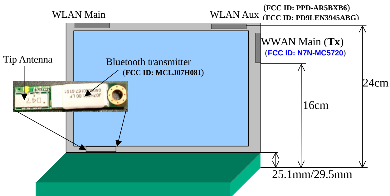
Figure-2 Antenna assembly of X60 series
