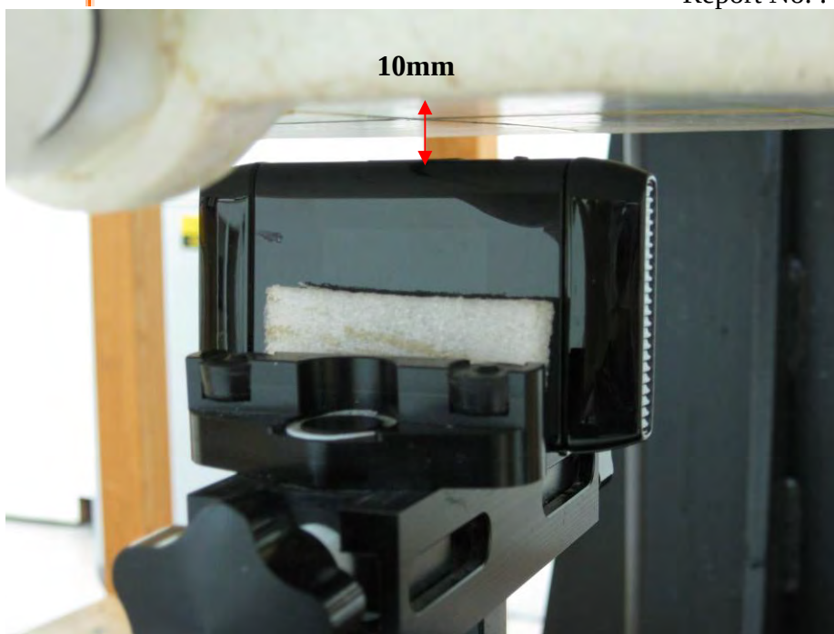
Fig.5 Top side.
