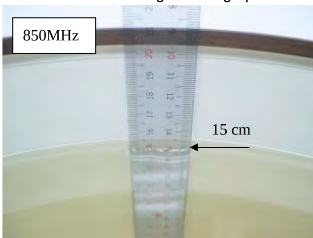
Fig.2.1 Photograph of the Tissue Simulant Fluid liquid depth 15cm for Flat (Body)
