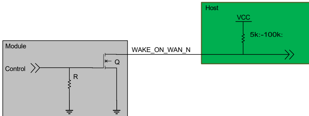
Figure 2-9: Recommended WAKE_ON_WAN_N host connection
