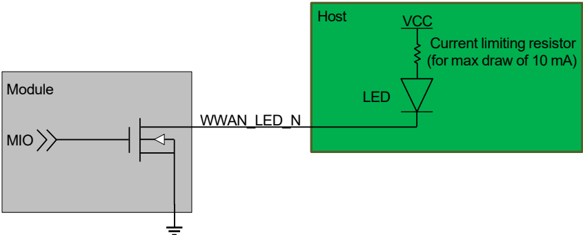
Figure 2-11: Recommended LED Connection
