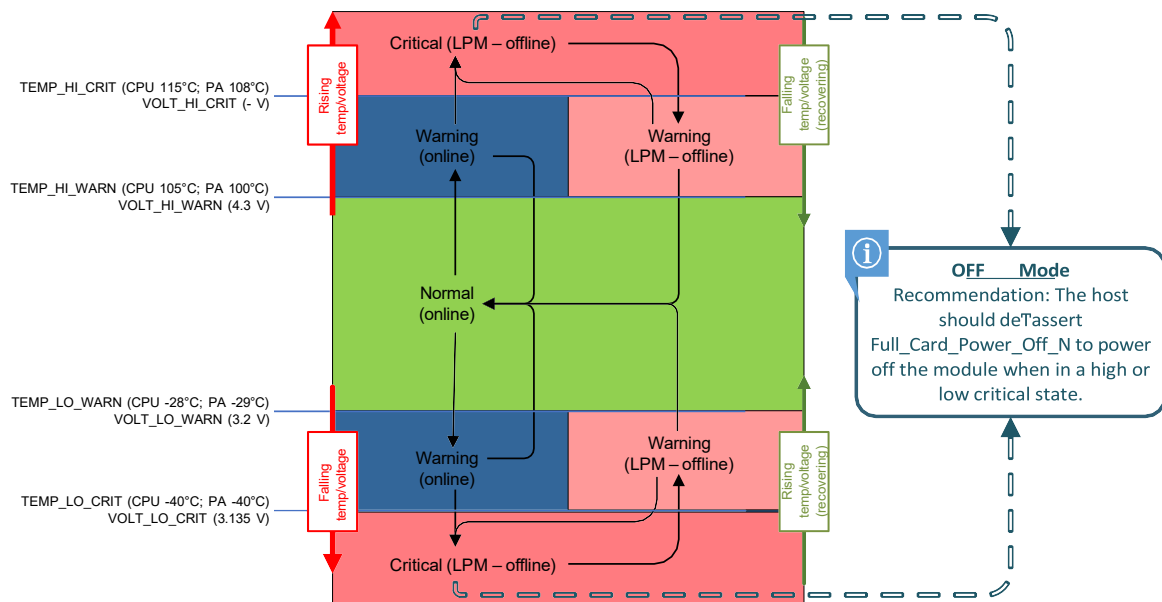
Figure 4-1: Voltage/Temperature Monitoring State Machines
