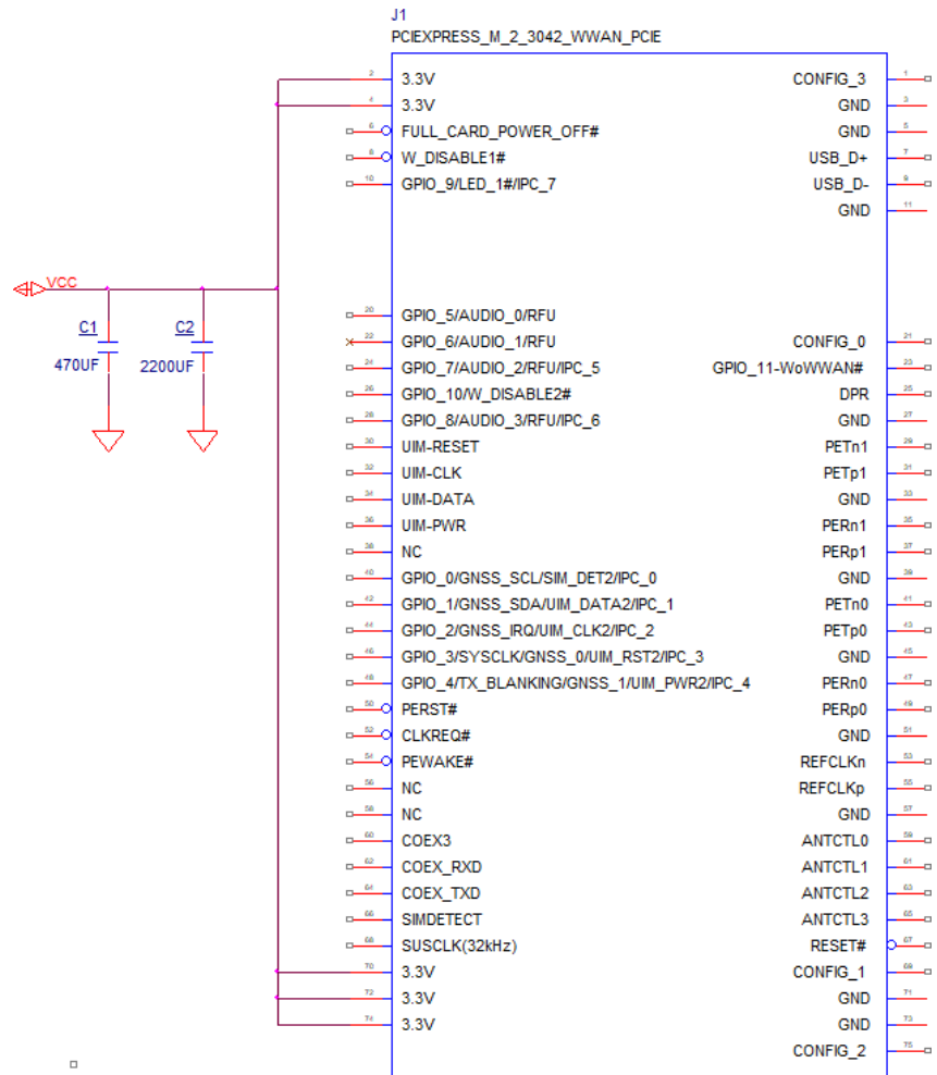
Figure 2-3: M.2 module VCC pins
