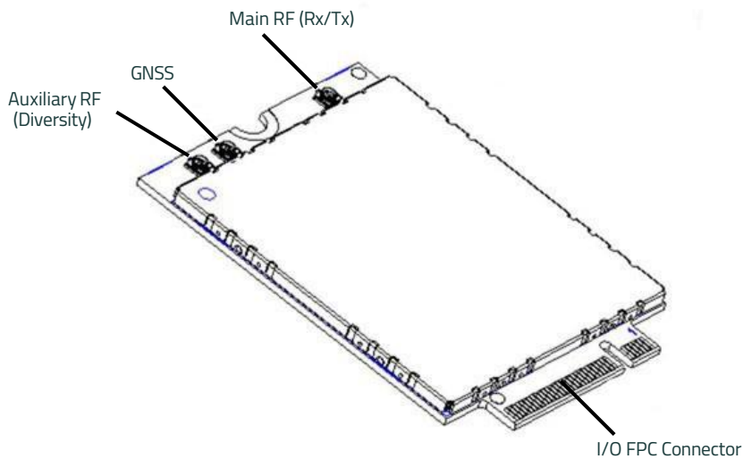
Figure 3-1: Module Connectors
