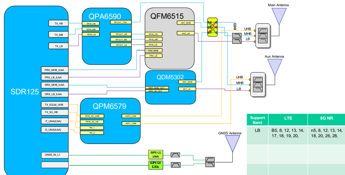
Figure 2-2: RF Block Diagram
