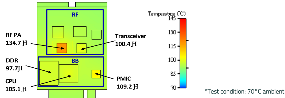
Figure 6-2: EM8695 Thermal Characteristics
