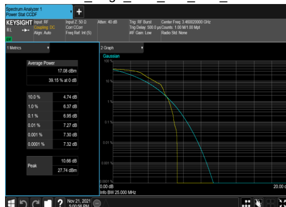
B5_N77(20M)_DFT-s-OFDM_PI_2- BPSK_Edge_1RB_Left_Low_CH
