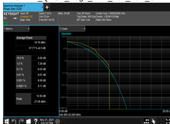
B5_N77(20M)_DFT-s- OFDM_QPSK_Edge_1RB_Left_Low_CH
