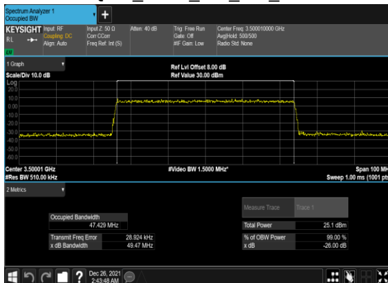
B5_N77(50M)_CP-OFDM_16 QAM_Outer_Full_Mid_CH
