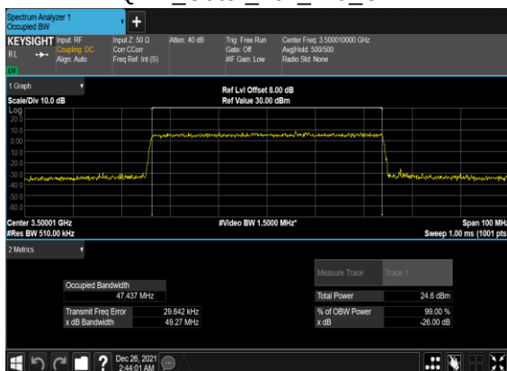
B5_N77(50M)_CP-OFDM_64 QAM_Outer_Full_Mid_CH
