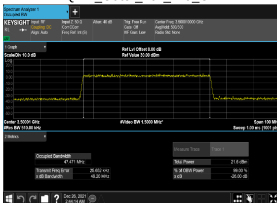
B5_N77(50M)_CP-OFDM_256 QAM_Outer_Full_Mid_CH
