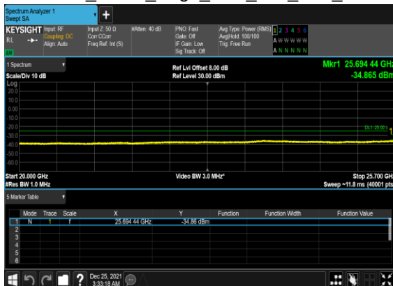
B5_N7(10M)_DFT-s- OFDM_BPSK_Edge_1RB_Left_Low_CH
