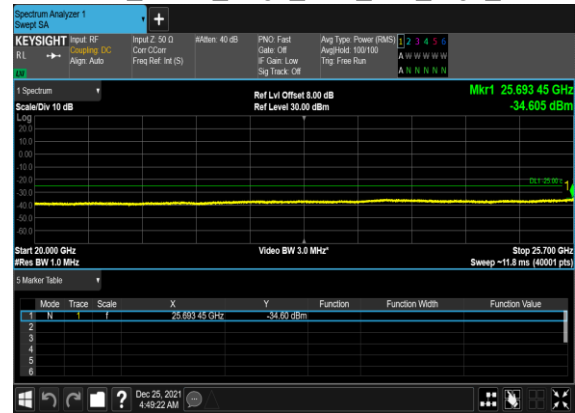
B5_N7(20M)_DFT-s- OFDM_BPSK_Edge_1RB_Left_High_CH
