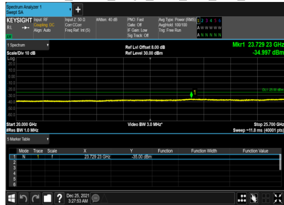
B5_N7(5M)_DFT-s- OFDM_BPSK_Edge_1RB_Left_Mid_CH
