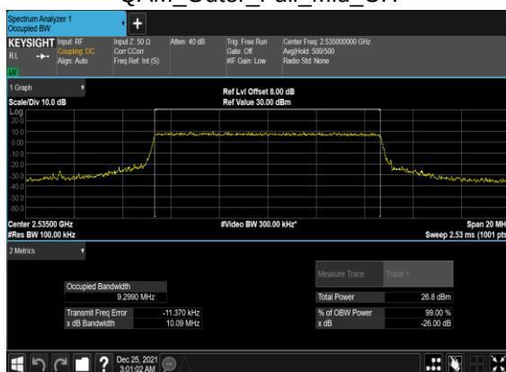
B5_N7(10M)_CP-OFDM_64 QAM_Outer_Full_Mid_CH
