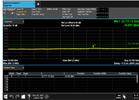
B5_N7(10M)_DFT-s- OFDM_BPSK_Edge_1RB_Left_High_CH
