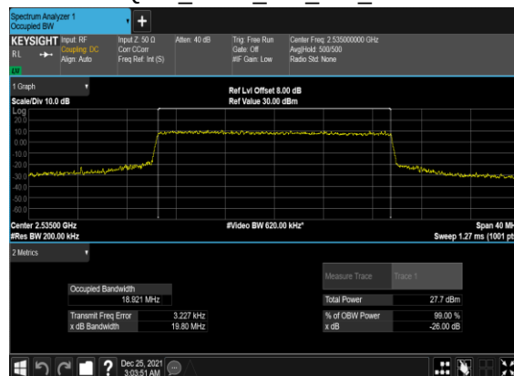
B5_N7(20M)_CP-OFDM_16 QAM_Outer_Full_Mid_CH
