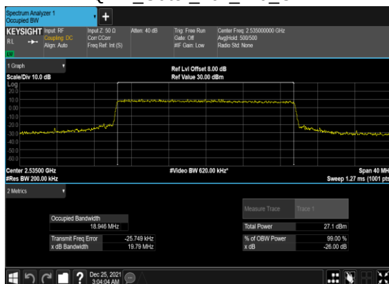
B5_N7(20M)_CP-OFDM_64 QAM_Outer_Full_Mid_CH
