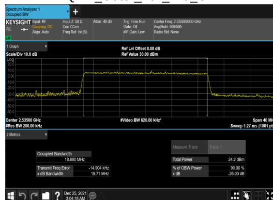
B5_N7(20M)_CP-OFDM_256 QAM_Outer_Full_Mid_CH
