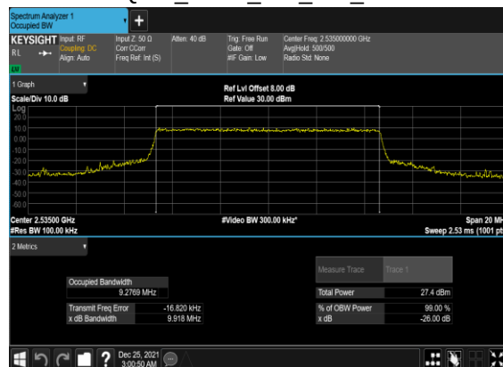
B5_N7(10M)_CP-OFDM_16 QAM_Outer_Full_Mid_CH
