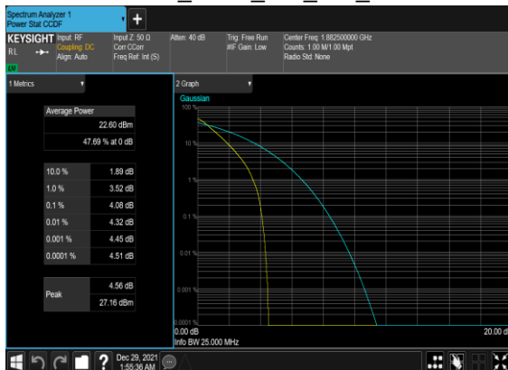
B12_N25(20M)_DFT-s-OFDM_PI_2- BPSK_Outer_Full_Mid_CH
