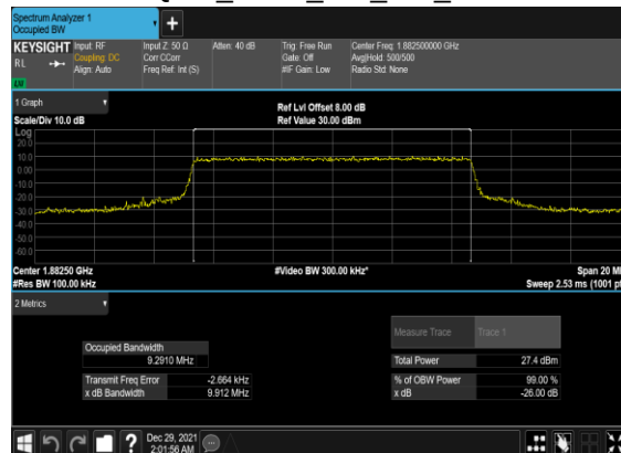
B12_N25(10M)_CP-OFDM_16 QAM_Outer_Full_Mid_CH
