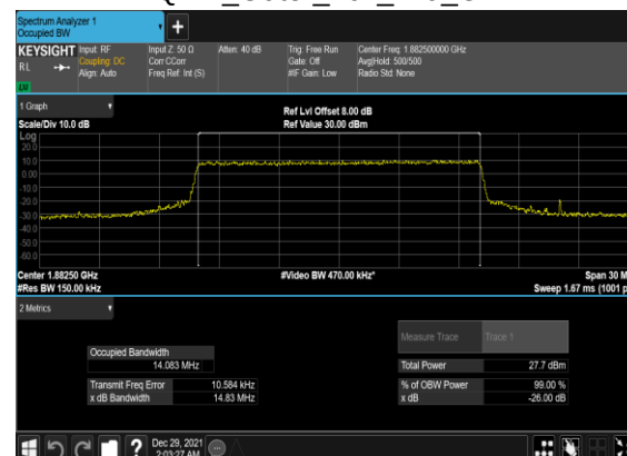
B12_N25(15M)_CP-OFDM_16 QAM_Outer_Full_Mid_CH
