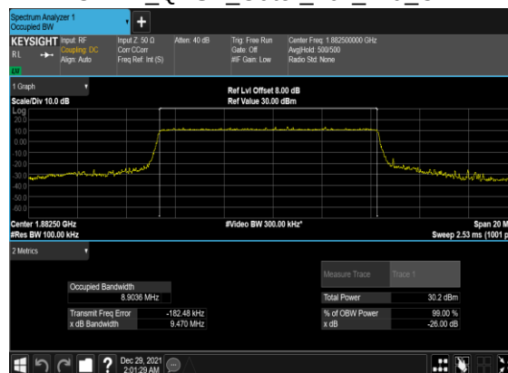
B12_N25(10M)_DFT-s- OFDM_QPSK_Outer_Full_Mid_CH
