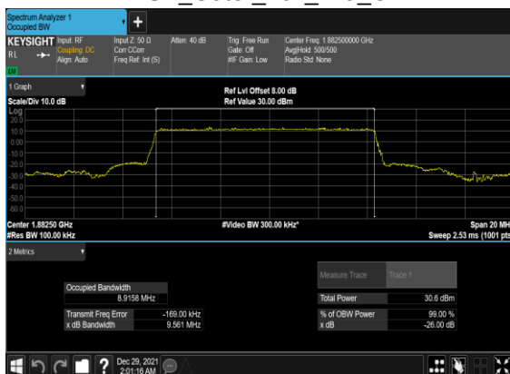
B12_N25(10M)_DFT-s-OFDM_PI_2- BPSK_Outer_Full_Mid_CH
