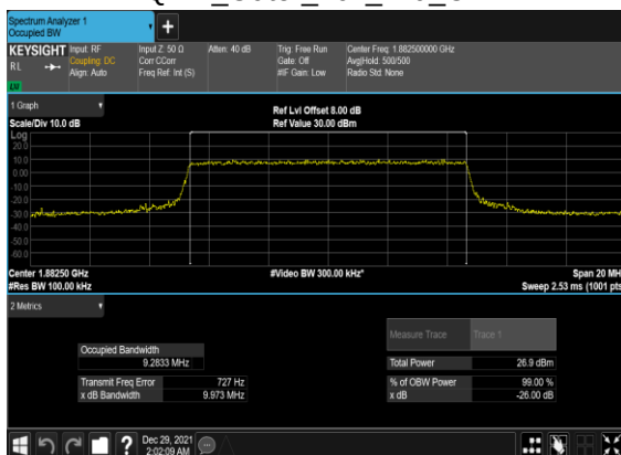
B12_N25(10M)_CP-OFDM_64 QAM_Outer_Full_Mid_CH
