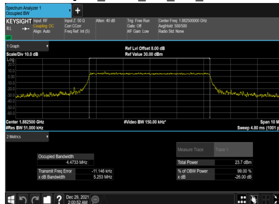
B12_N25(5M)_CP-OFDM_256 QAM_Outer_Full_Mid_CH
