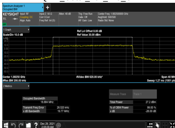
B12_N25(20M)_CP-OFDM_64 QAM_Outer_Full_Mid_CH
