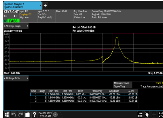
B12_N25(10M)_DFT-s- OFDM_QPSK_Edge_1RB_Left_Low_CH
