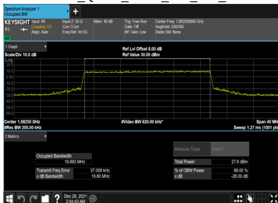
B12_N25(20M)_CP- OFDM_QPSK_Outer_Full_Mid_CH
