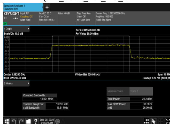
B12_N25(20M)_CP-OFDM_256 QAM_Outer_Full_Mid_CH
