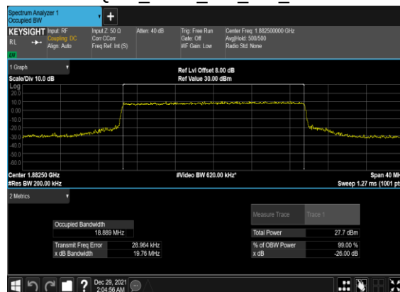
B12_N25(20M)_CP-OFDM_16 QAM_Outer_Full_Mid_CH
