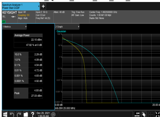
B12_N25(20M)_DFT-s- OFDM_QPSK_Outer_Full_Mid_CH
