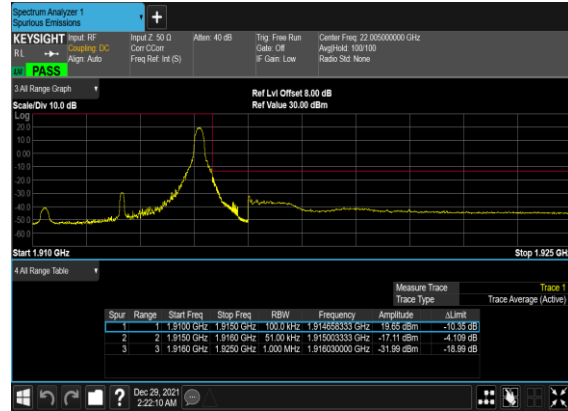
B12_N25(5M)_DFT-s- OFDM_QPSK_Edge_1RB_Right_High_CH
