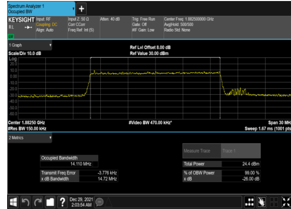
B12_N25(15M)_CP-OFDM_256 QAM_Outer_Full_Mid_CH
