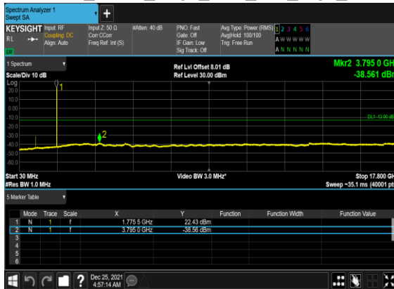
B13_N66(5M)_DFT-s- OFDM_BPSK_Edge_1RB_Left_High_CH
