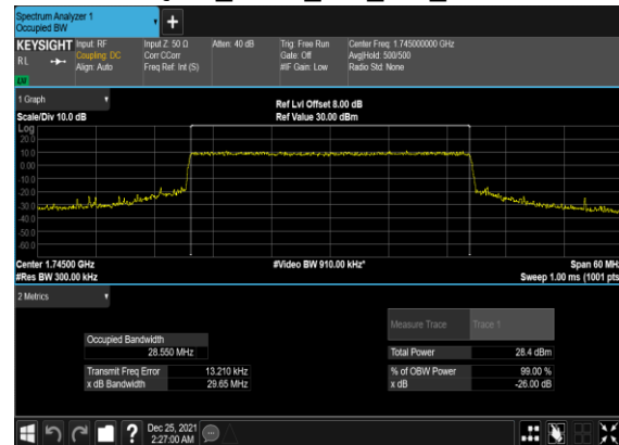
B13_N66(30M)_CP-OFDM_16 QAM_Outer_Full_Mid_CH
