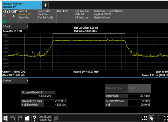
B13_N66(5M)_DFT-s-OFDM_PI_2- BPSK_Outer_Full_Mid_CH
