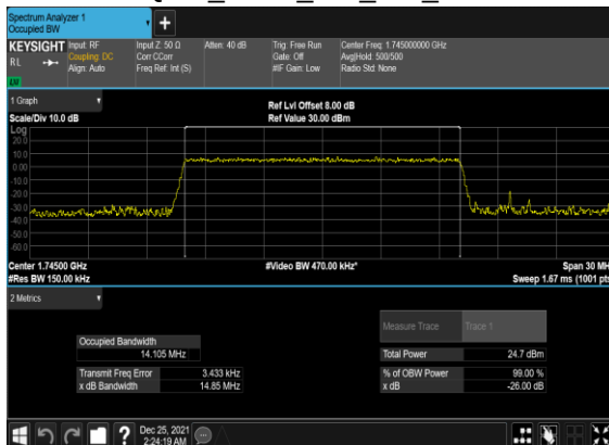
B13_N66(15M)_CP-OFDM_256 QAM_Outer_Full_Mid_CH
