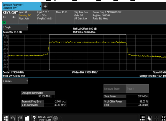
B13_N66(40M)_CP- OFDM_QPSK_Outer_Full_Mid_CH
