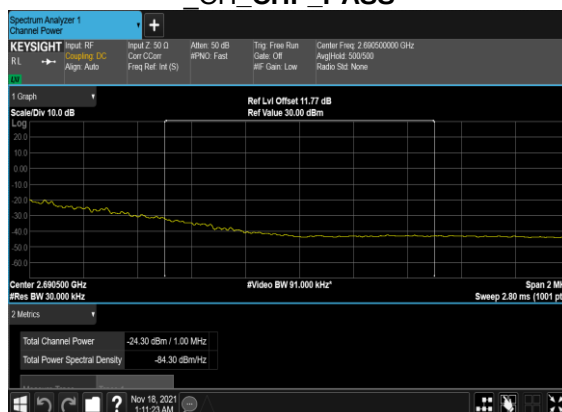
B4_N41(100M)_DFT-s- OFDM_BPSK_Edge_1RB_Right_High CH_CHP_PASS
