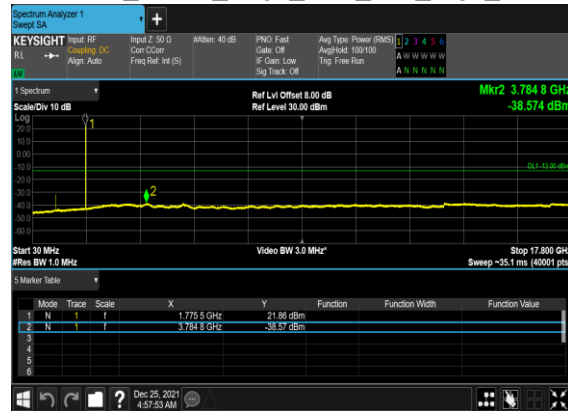
B13_N66(5M)_DFT-s- OFDM_QPSK_Edge_1RB_Left_High_CH
