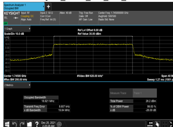
B13_N66(20M)_CP-OFDM_16 QAM_Outer_Full_Mid_CH
