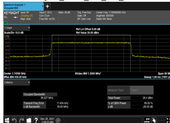
B13_N66(40M)_CP-OFDM_16 QAM_Outer_Full_Mid_CH
