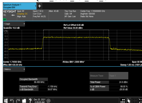
B13_N66(40M)_CP-OFDM_256 QAM_Outer_Full_Mid_CH
