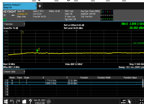
B13_N66(20M)_DFT-s- OFDM_QPSK_Edge_1RB_Left_Low_CH
