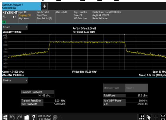
B13_N66(15M)_CP-OFDM_64 QAM_Outer_Full_Mid_CH
