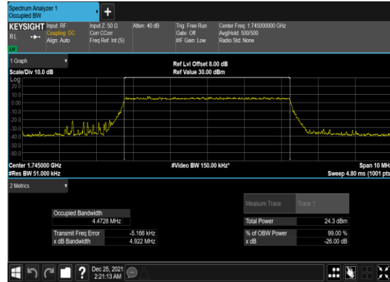
B13_N66(5M)_CP-OFDM_256 QAM_Outer_Full_Mid_CH
