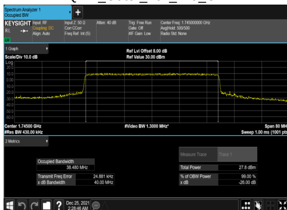
B13_N66(40M)_CP-OFDM_64 QAM_Outer_Full_Mid_CH
