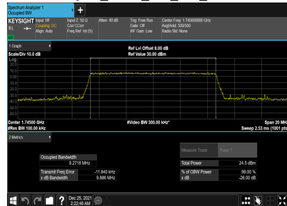
B13_N66(10M)_CP-OFDM_256 QAM_Outer_Full_Mid_CH
