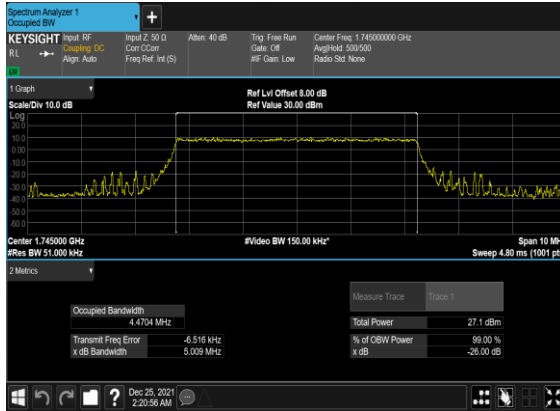
B13_N66(5M)_CP-OFDM_64 QAM_Outer_Full_Mid_CH
