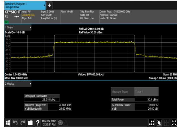
B13_N66(30M)_DFT-s- OFDM_QPSK_Outer_Full_Mid_CH
