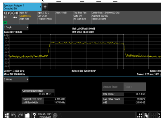
B13_N66(20M)_CP-OFDM_256 QAM_Outer_Full_Mid_CH
