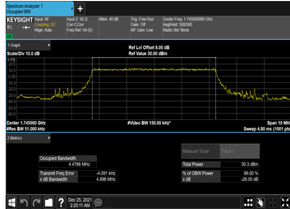
B13_N66(5M)_DFT-s- OFDM_QPSK_Outer_Full_Mid_CH
