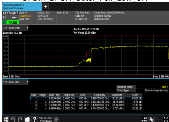
B4_N41(100M)_DFT-s- OFDM BPSK Outer Full Low CH
