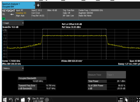
B13_N66(20M)_CP- OFDM_QPSK_Outer_Full_Mid_CH
