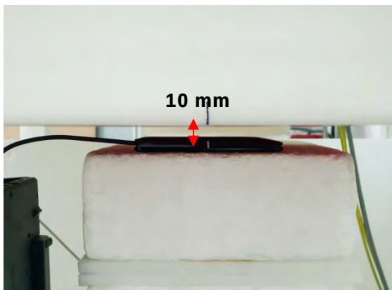
Fig.4 EUT Front side to flat phantom
