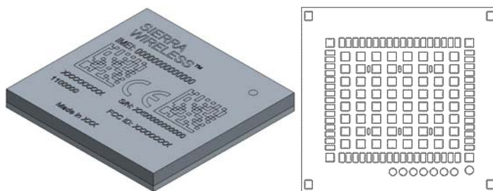
Figure 2. Mechanical Overview
