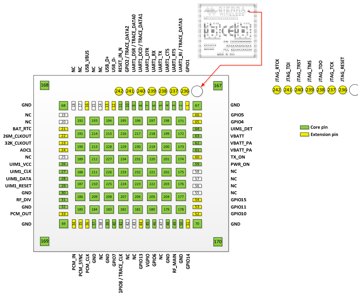
Figure 3. Pad Configuration
