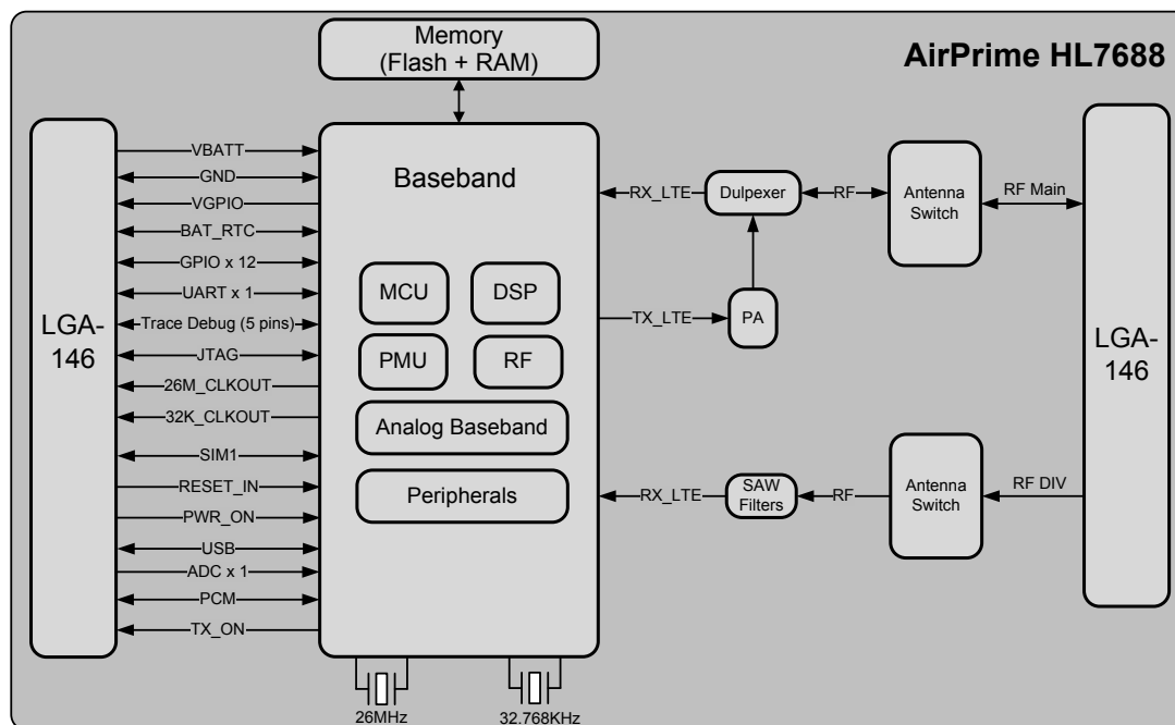
Figure 1. Architecture Overview
