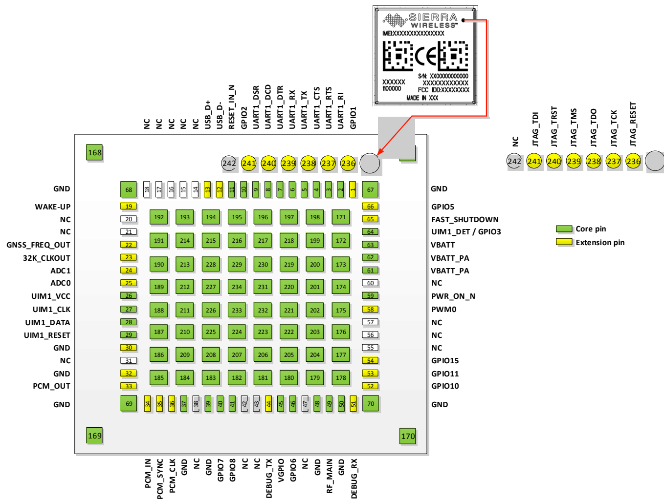
Figure 5. Pad Configuration
