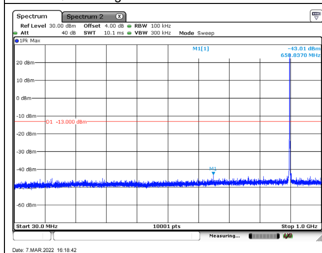
3 MHz / QPSK - Hight / CH21640 / 1RB5 / Below 1 GHz
