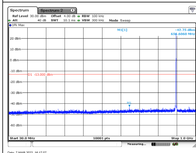
3 MHz / QPSK - Low / CH21640 / 1RB0 / Below 1 GHz
