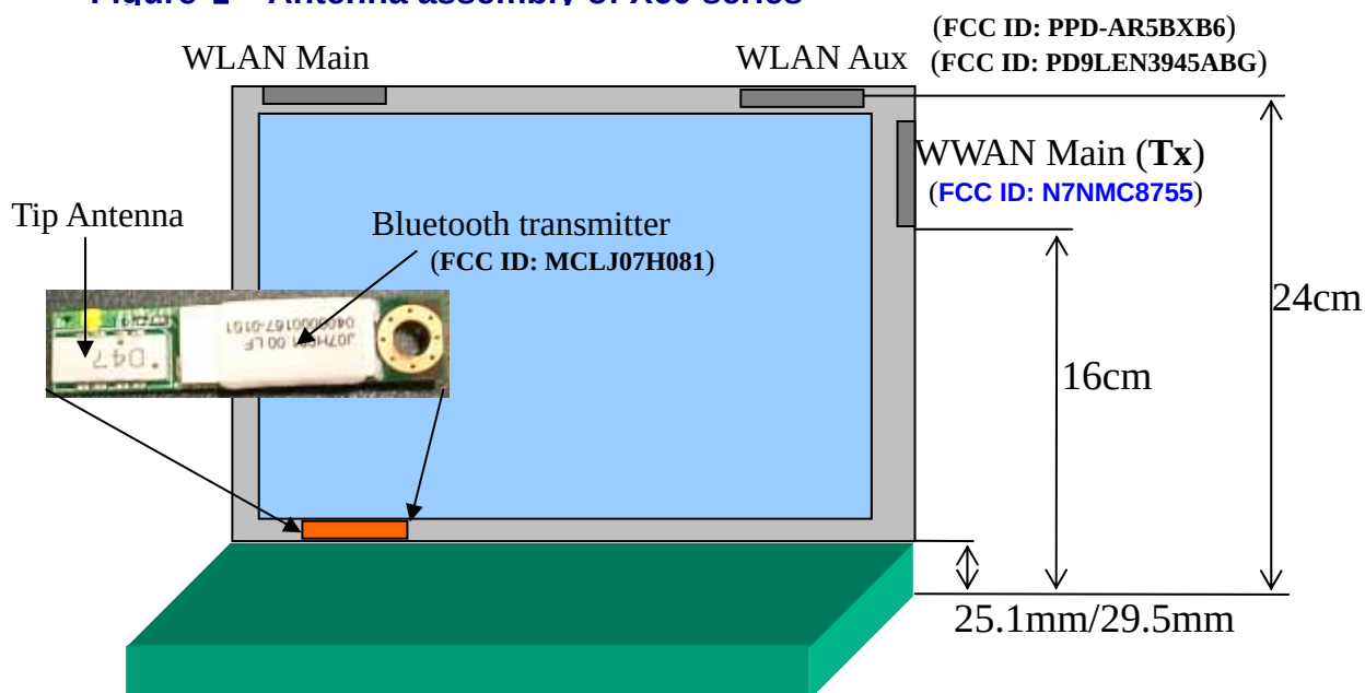
Figure-1 Antenna assembly of X60 series
