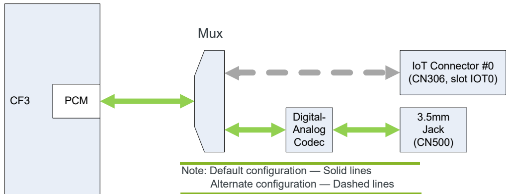
Figure 2-6: Audio Configuration
