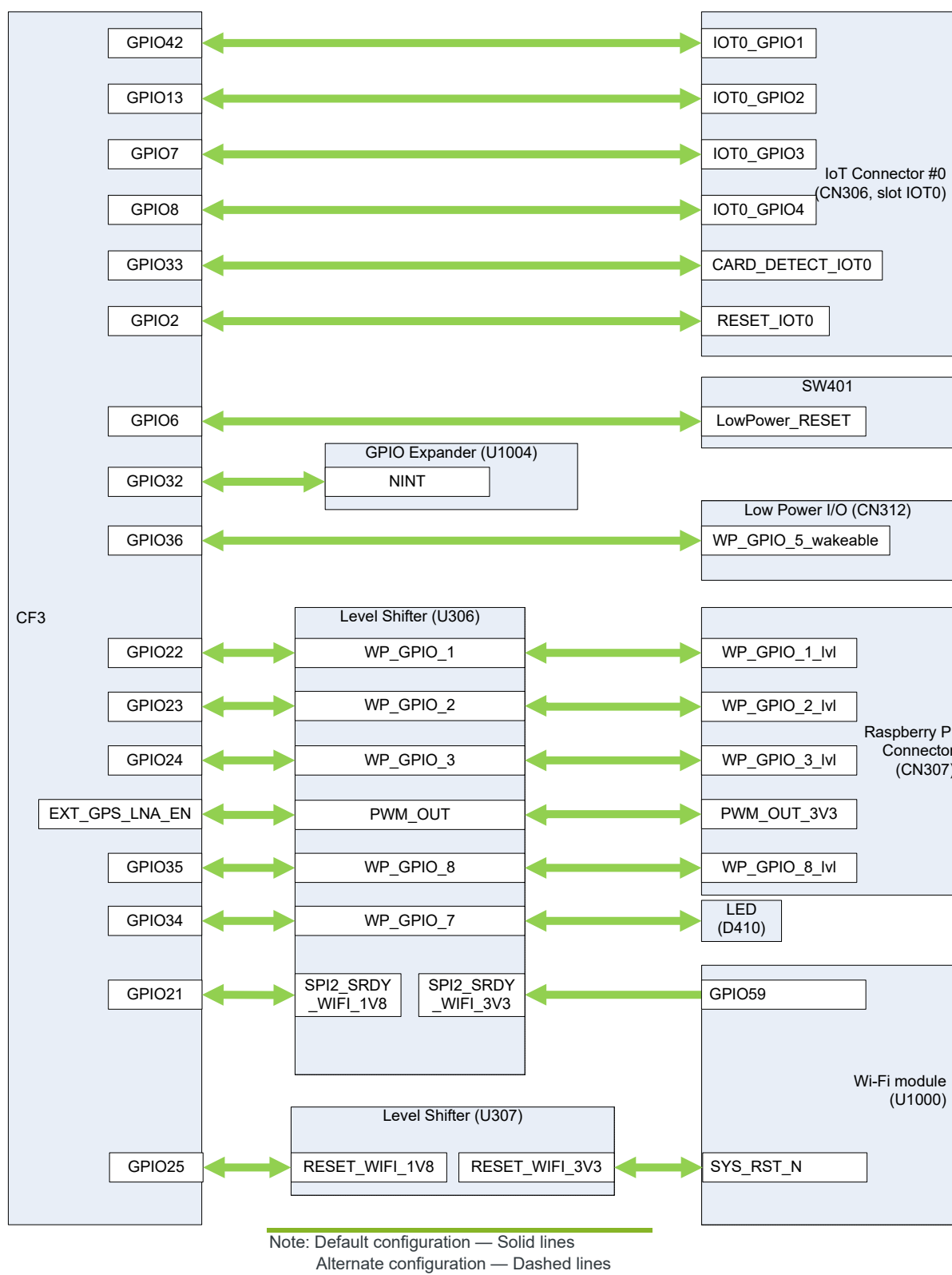
Figure 2-7: GPIO Configuration
