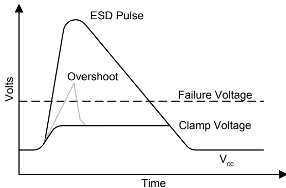
Figure 7-4: Possible inductance voltage overshoot
