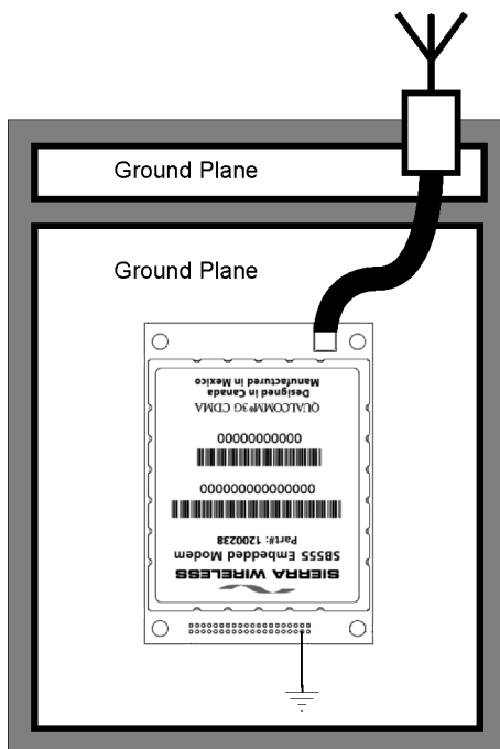
Figure 7-1: Ground plane RF Isolation
