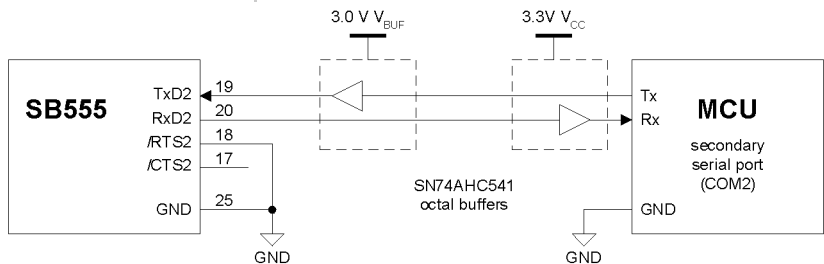
Figure 4-5: Secondary serial port minimum integration
