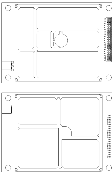
Figure 2-3: Shield fence frame
