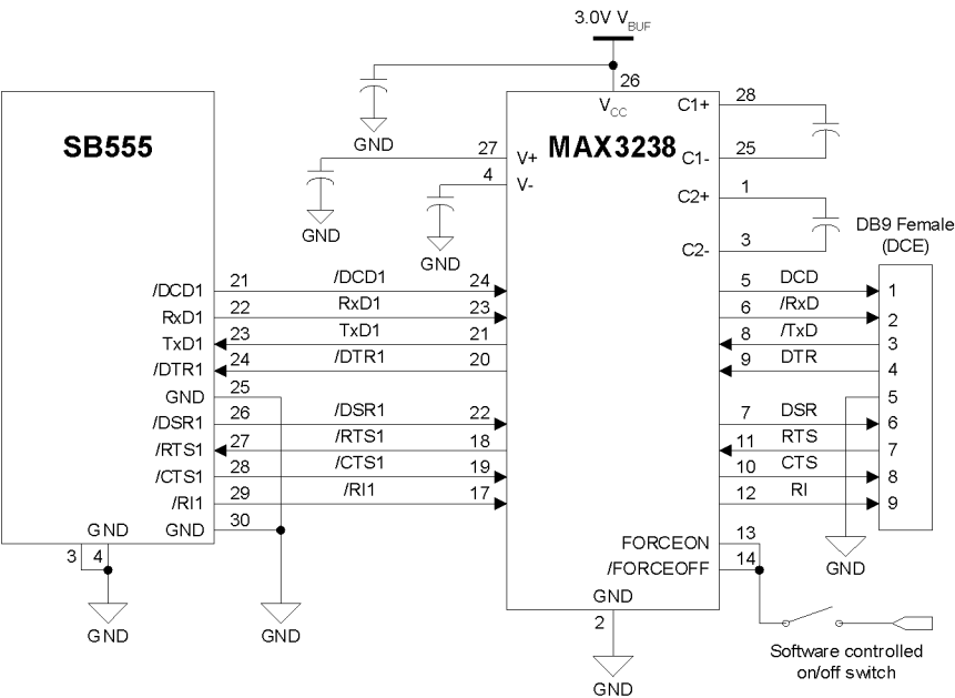
Figure 4-2: Primary serial port integration—external RS-232 connector
