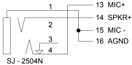
Figure 5-2: Sample headset integration
