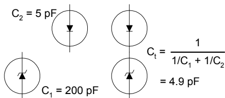
Figure 7-5: Reducing capacitance with rectifier
