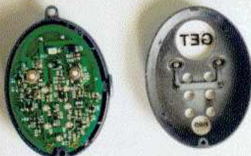
Photo-5: Front Cover Removed
