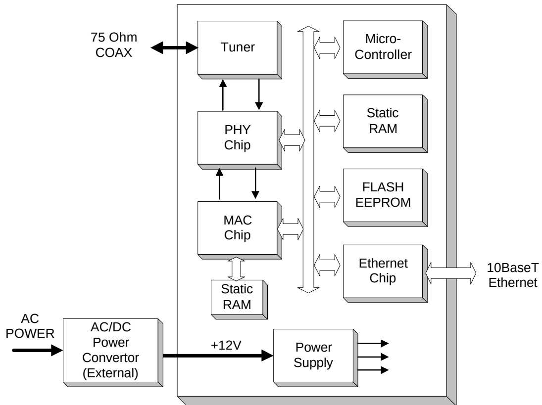
Block diagram of External cable modem
