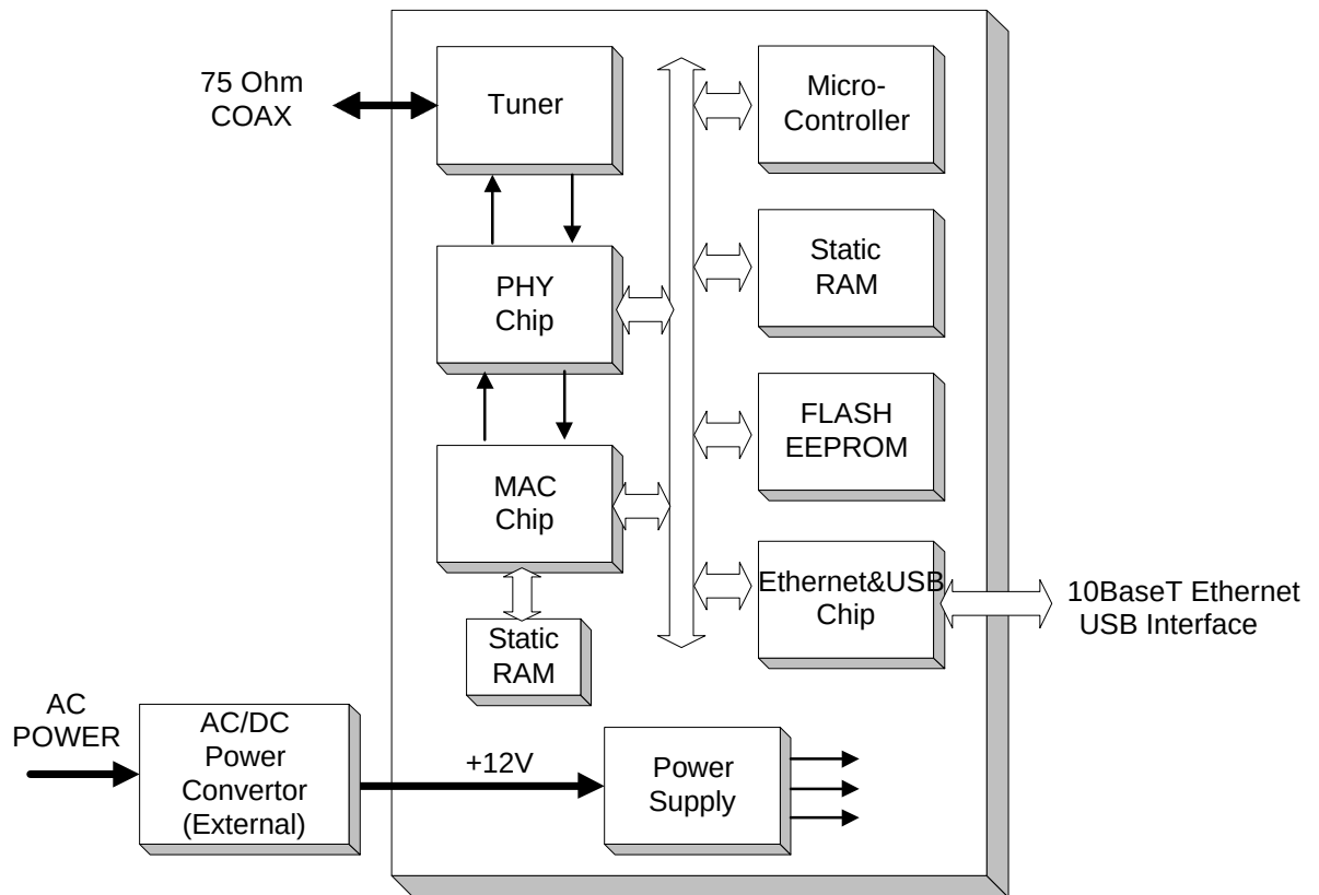
Block diagram of External cable modem
